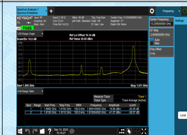
Band2-15MHz-16QAM-19125-1RB#74-PASS
