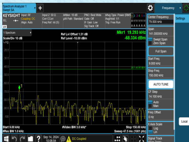
Band2-5MHz-QPSK-19175-1RB#0-0.009~0.15-PASS
