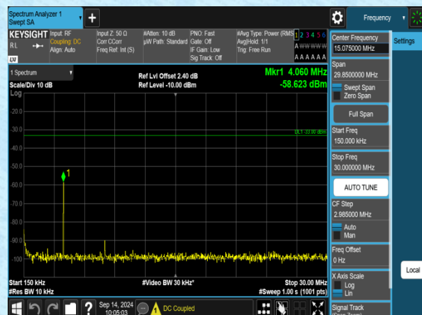
Band2-5MHz-QPSK-18625-1RB#0-0.15~30-PASS
