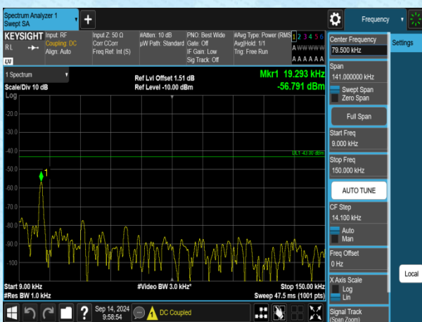
Band2-3MHz-QPSK-18900-1RB#0-0.009~0.15-PASS
