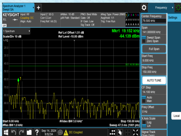
Band2-1.4MHz-QPSK-19193-1RB#0-0.009~0.15-PASS
