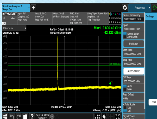
Band2-5MHz-QPSK-18900-1RB#0-1000~3000-PASS
