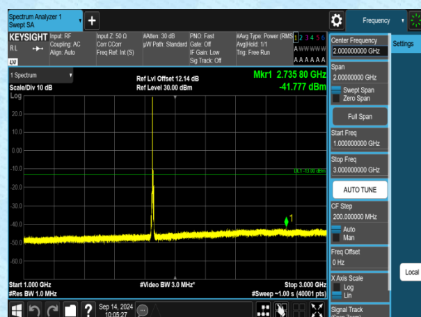
Band2-5MHz-QPSK-18625-1RB#0-1000~3000-PASS
