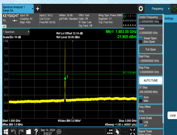
Band2-1.4MHz-QPSK-18900-1RB#0-1000~3000-PASS
