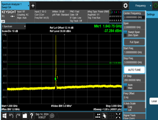
Band2-3MHz-QPSK-18615-1RB#0-1000~3000-PASS
