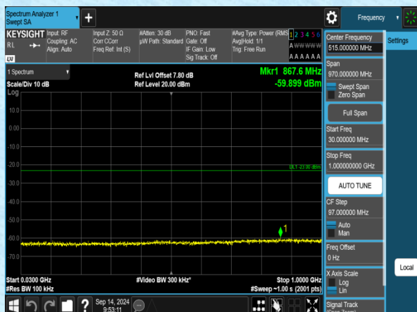
Band2-1.4MHz-QPSK-19193-1RB#0-30~1000-PASS
