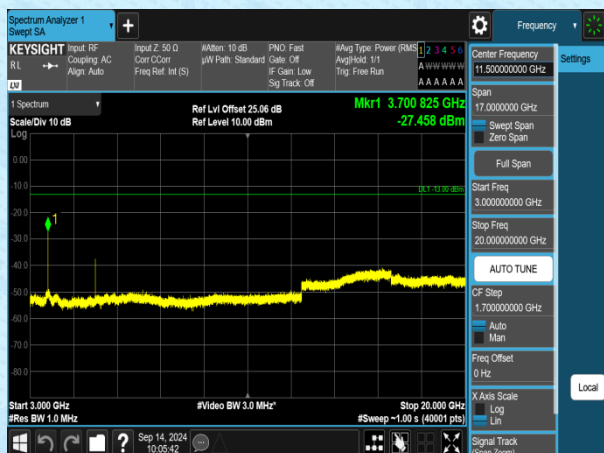
Band2-5MHz-QPSK-18625-1RB#0-3000~20000-PASS
