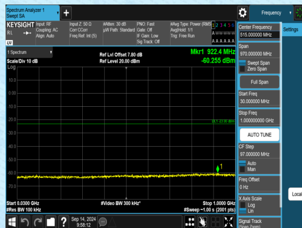
Band2-3MHz-QPSK-18615-1RB#0-30~1000-PASS
