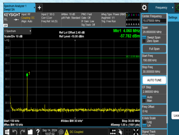
Band2-5MHz-QPSK-19175-1RB#0-0.15~30-PASS
