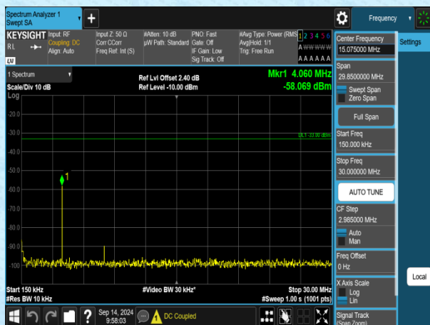
Band2-3MHz-QPSK-18615-1RB#0-0.15~30-PASS
