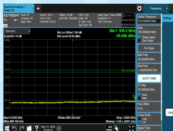
Band2-3MHz-QPSK-19185-1RB#0-30~1000-PASS
