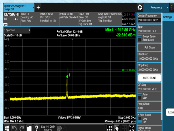
Band2-1.4MHz-QPSK-19193-1RB#0-1000~3000-PASS
