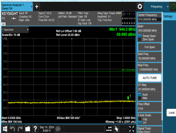
Band2-3MHz-QPSK-18900-1RB#0-30~1000-PASS
