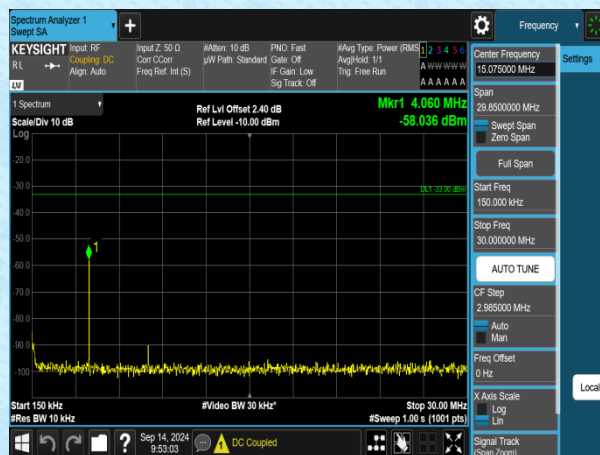
Band2-1.4MHz-QPSK-19193-1RB#0-0.15~30-PASS
