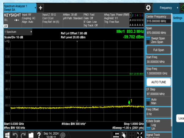
Band2-5MHz-QPSK-18900-1RB#0-30~1000-PASS
