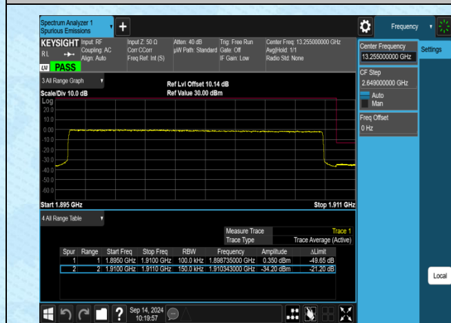
Band2-15MHz-16QAM-19125-75RB#0-PASS
