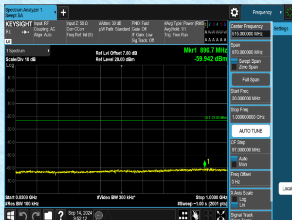
Band2-1.4MHz-QPSK-18900-1RB#0-30~1000-PASS
