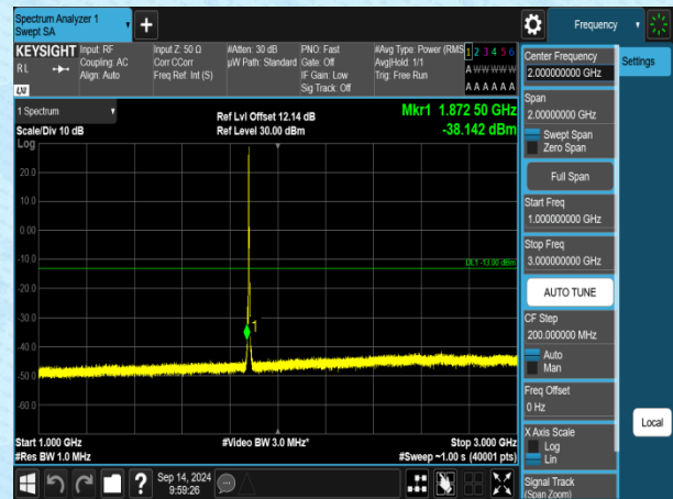
Band2-3MHz-QPSK-18900-1RB#0-1000~3000-PASS
