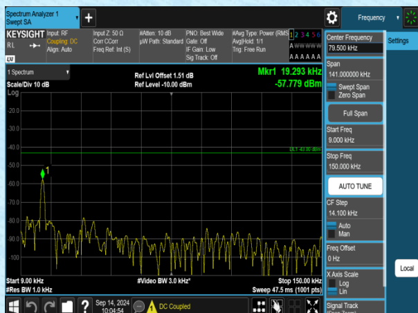
Band2-5MHz-QPSK-18625-1RB#0-0.009~0.15-PASS
