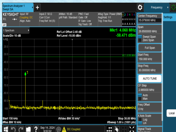
Band2-1.4MHz-QPSK-18900-1RB#0-0.15~30-PASS
