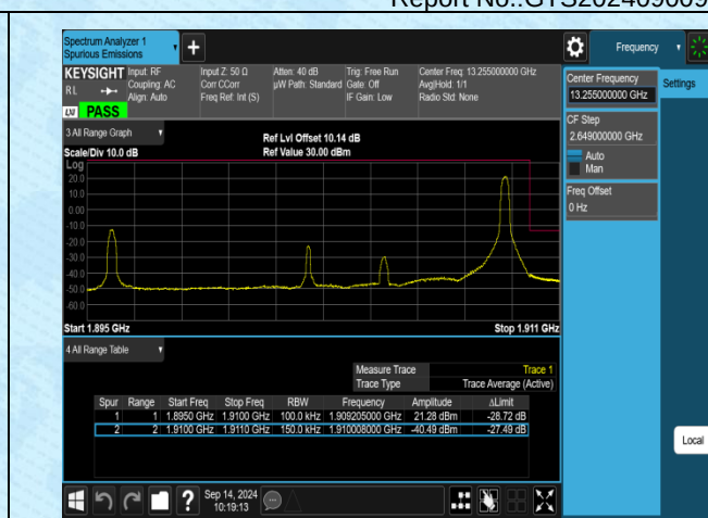
Band2-15MHz-QPSK-19125-1RB#74-PASS
