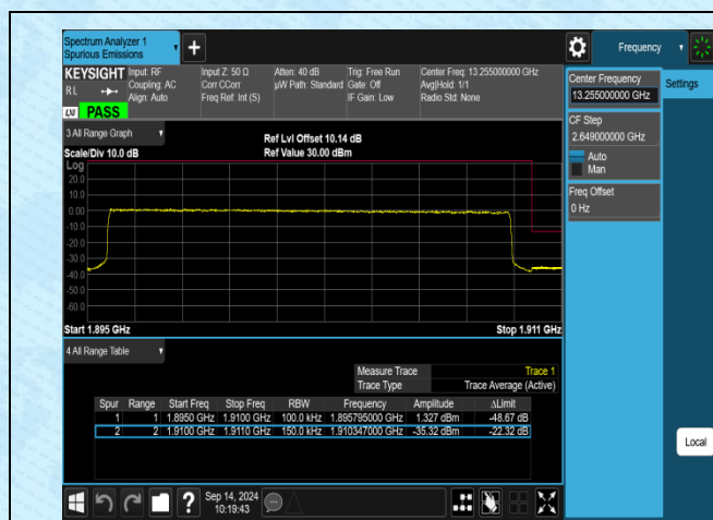
Band2-15MHz-QPSK-19125-75RB#0-PASS
