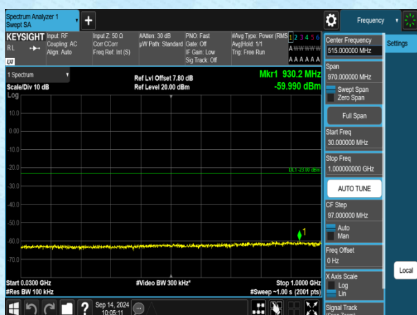
Band2-5MHz-QPSK-18625-1RB#0-30~1000-PASS
