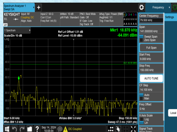
Band2-5MHz-QPSK-18900-1RB#0-0.009~0.15-PASS
