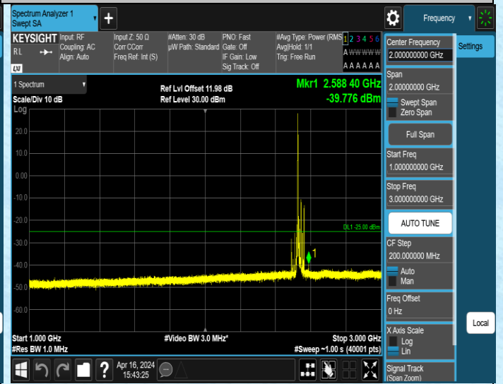
Band7_20MHz_QPSK_21100_1RB#0_1000~3000_1000~3000 0
