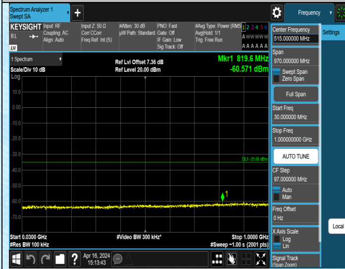
Band7_20MHz_QPSK_21100_1RB#0_30~1000_30~1000
