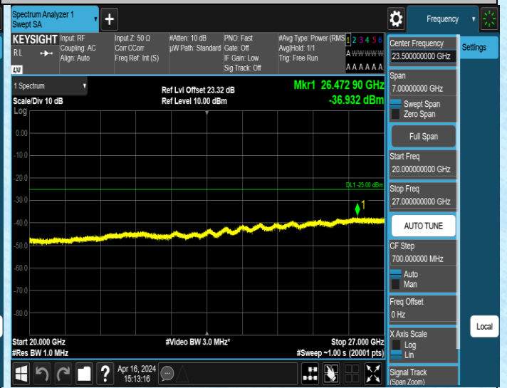
Band7_20MHz_QPSK_20850_1RB#0_20000~27000_20000~ 27000
