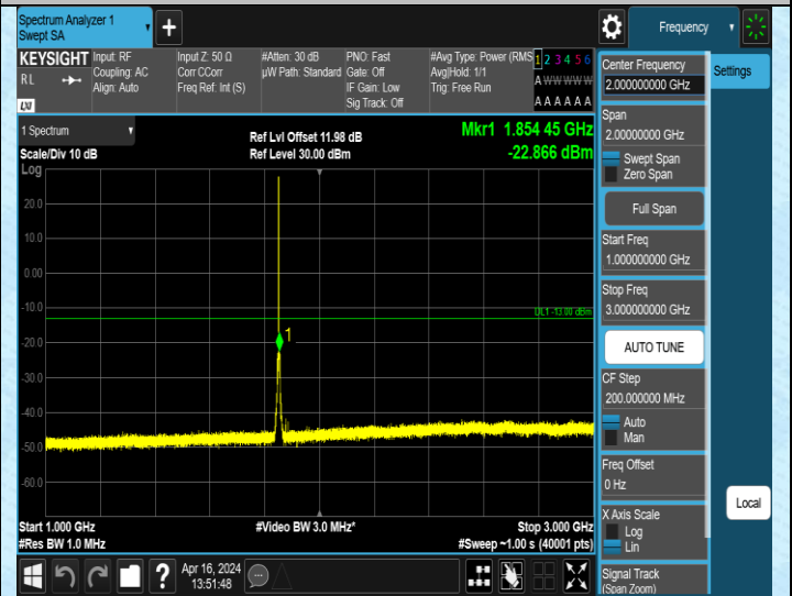
Band2_1.4MHz_QPSK_18607_1RB#0_1000~3000_1000~3000
