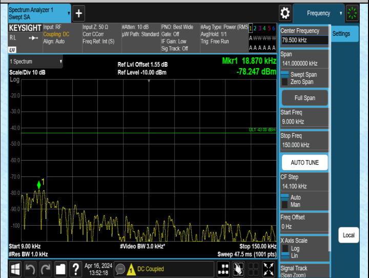
Band2_1.4MHz_QPSK_18900_1RB#0_0.009~0.15_0.009~0.15
