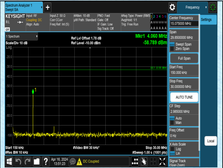
Band2_1.4MHz_QPSK_18607_1RB#0_0.15~30_0.15~30
