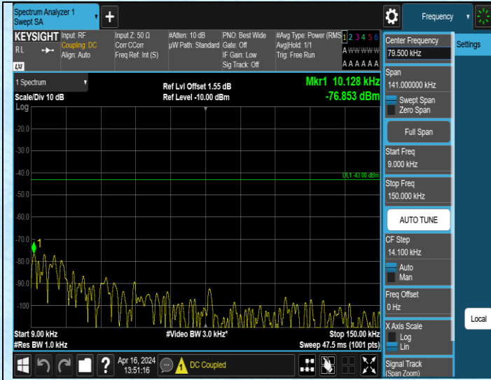
Band2_1.4MHz_QPSK_18607_1RB#0_0.009~0.15_0.009~0.15
