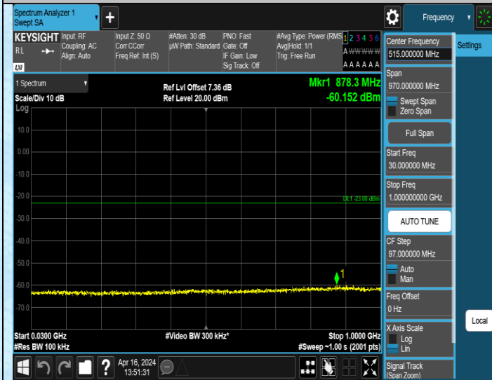
Band2_1.4MHz_QPSK_18607_1RB#0_30~1000_30~1000
