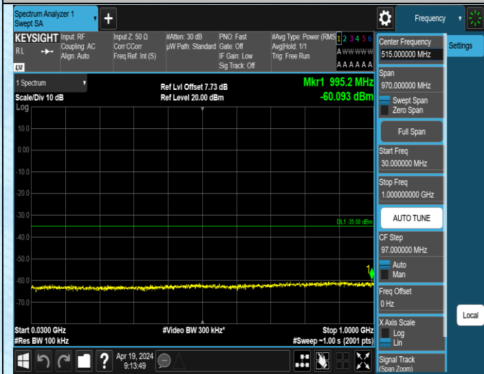
Band41_20MHz_QPSK_40140_1RB#0_30~1000_30~1000
