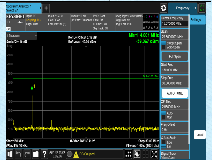
Band41_10MHz_QPSK_40090_1RB#0_0.15~30_0.15~30
