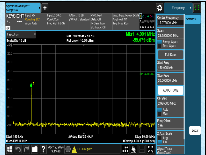
Band41_20MHz_QPSK_40140_1RB#0_0.15~30_0.15~30
