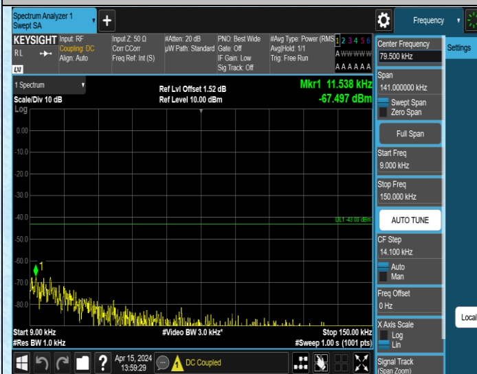
Band2-9538-0.009~0.15MHz-PASS
