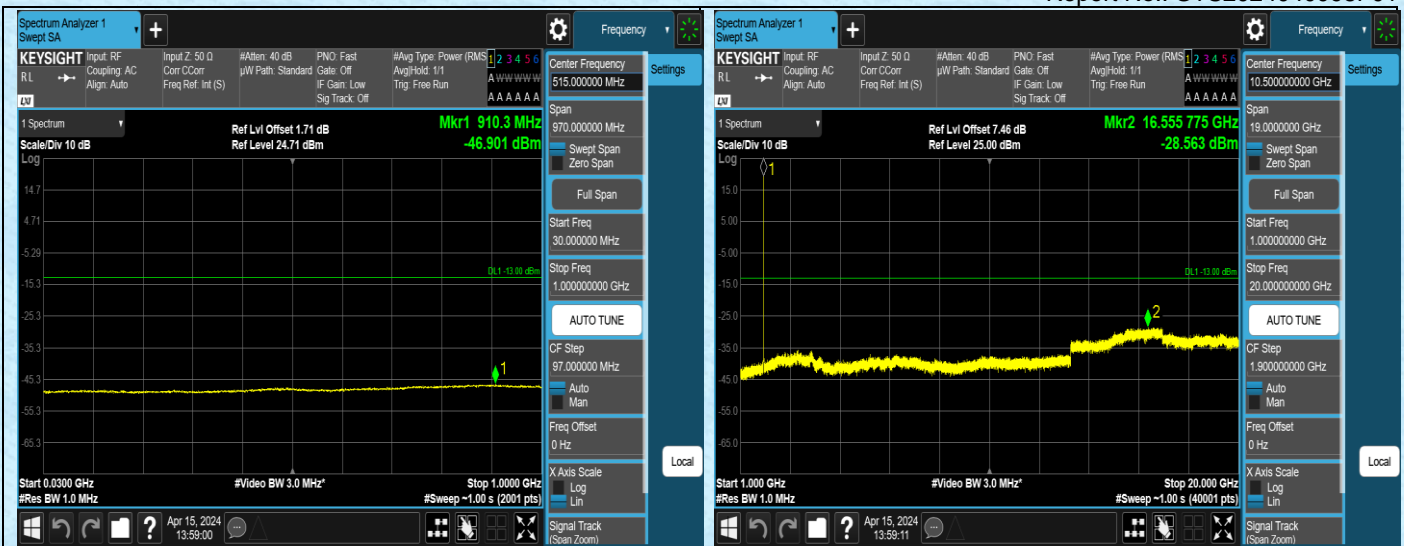
Band2-9400-30~1000MHz-PASS
