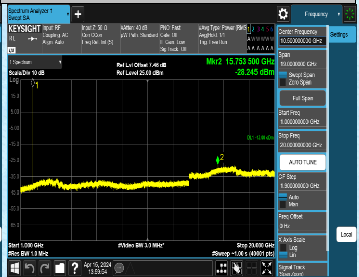
Band2-9538-1000~20000MHz-PASS
