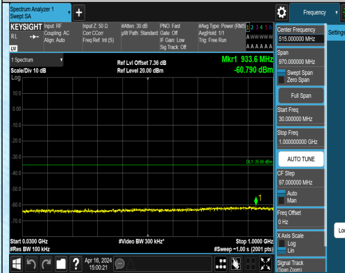
Band7_5MHz_QPSK_20775_1RB#0_30~1000_30~1000
