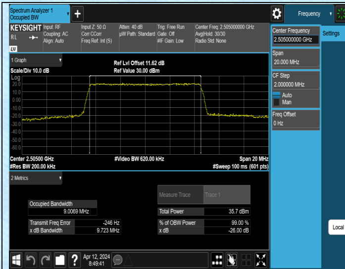
Band7-10MHz-QPSK-20800-50RB#0-PASS
