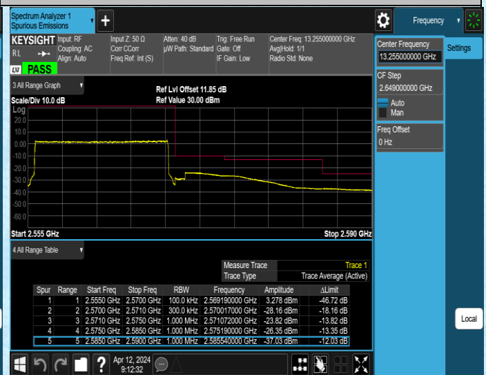
Band7_15MHz_QPSK_21375_75RB#0
