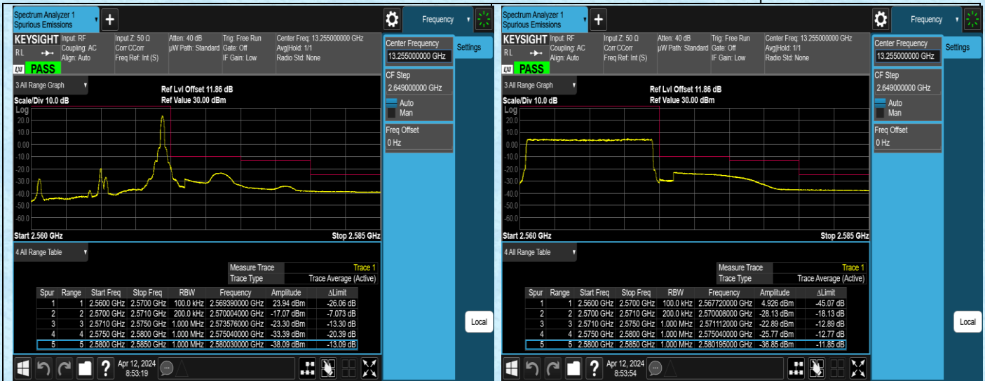
Band7_10MHz_QPSK_21400_1RB#49
