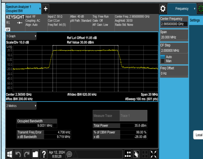
Band7-10MHz-QPSK-21400-50RB#0-PASS
