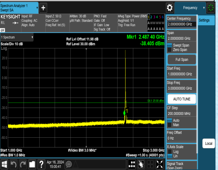
Band7_5MHz_QPSK_20775_1RB#0_1000~3000_1000~3000
