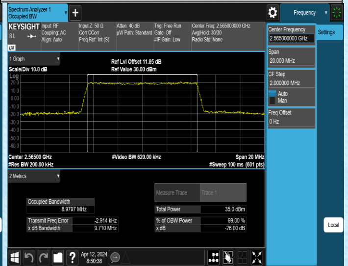
Band7-10MHz-16QAM-21400-50RB#0-PASS
