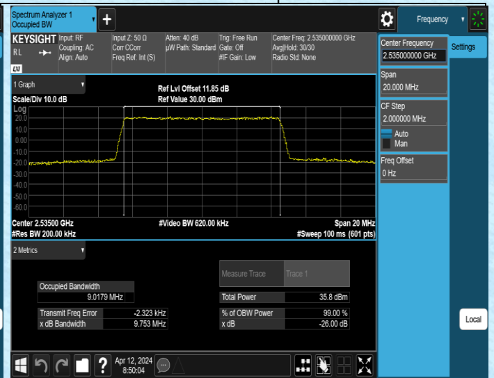
Band7-10MHz-QPSK-21100-50RB#0-PASS
