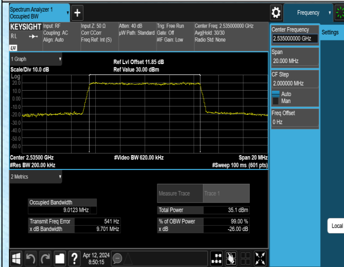
Band7-10MHz-16QAM-21100-50RB#0-PASS
