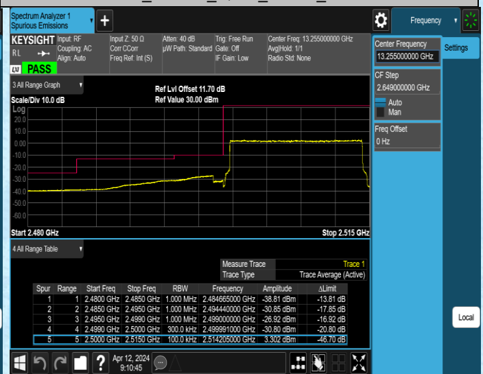
Band7_15MHz_QPSK_20825_75RB#0
