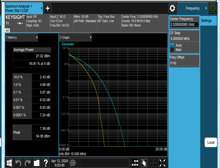
Band7-15MHz-QPSK-21100-75RB#0-PASS
