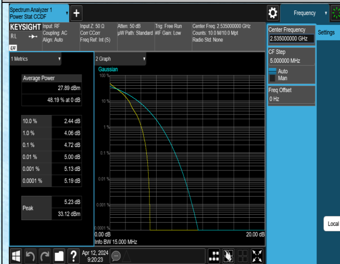
Band7-15MHz-QPSK-21100-1RB#0-PASS
