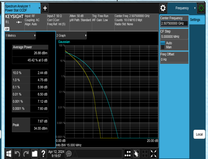
Band7-15MHz-QPSK-20825-75RB#0-PASS
