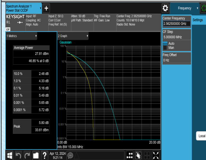
Band7-15MHz-QPSK-21375-1RB#0-PASS
