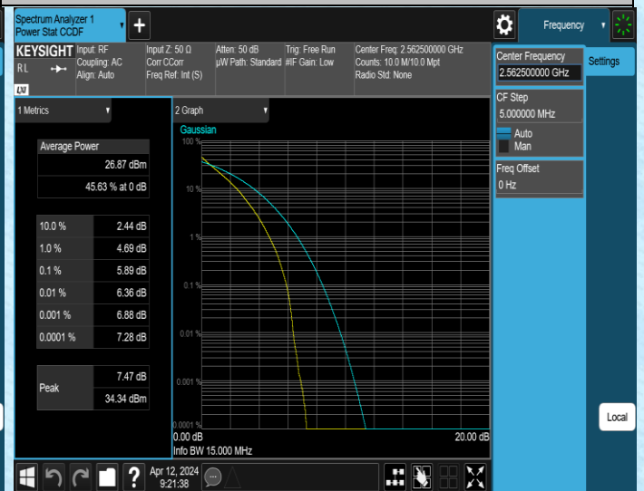
Band7-15MHz-QPSK-21375-75RB#0-PASS
