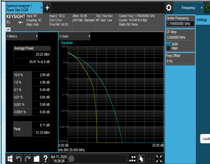
Band4-20MHz-QPSK-20300-1RB#0-PASS
