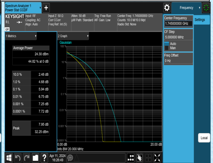
Band4-20MHz-QPSK-20300-100RB#0-PASS
