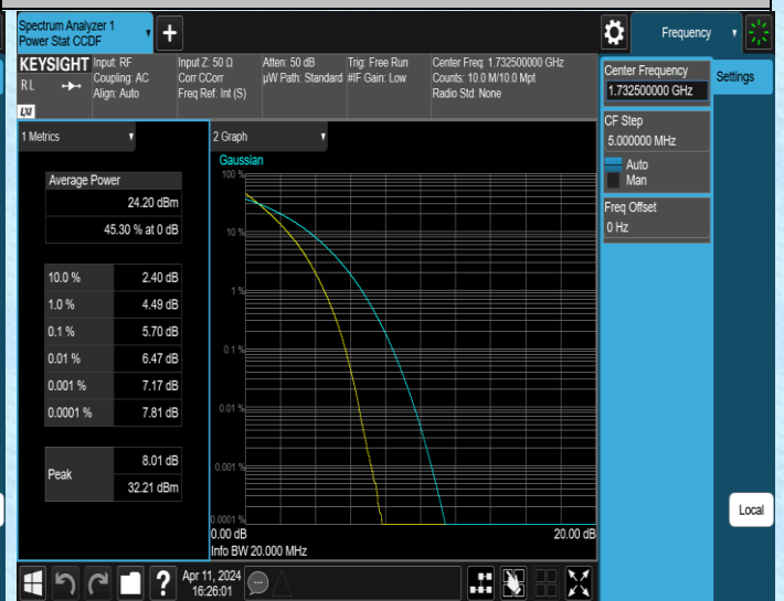
Band4-20MHz-QPSK-20175-100RB#0-PASS
