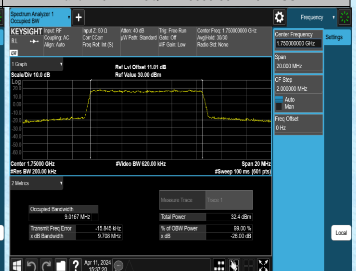
Band4-10MHz-16QAM-20350-50RB#0-PASS
