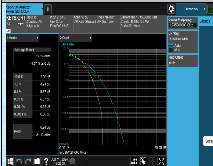
Band4-20MHz-16QAM-20300-1RB#0-PASS
