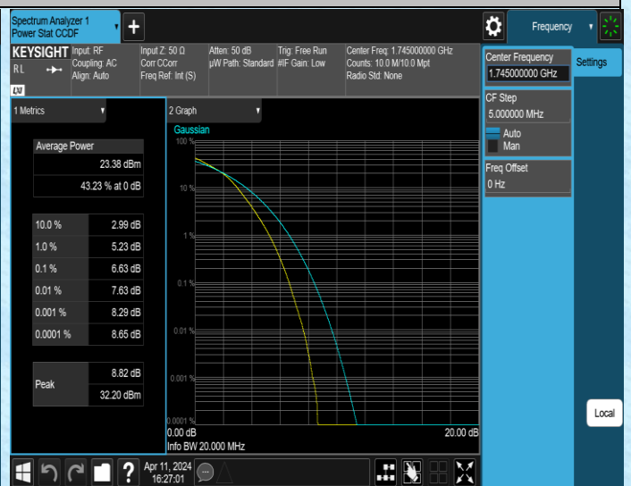
Band4-20MHz-16QAM-20300-100RB#0-PASS
