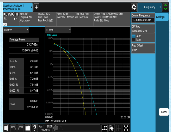
Band4-20MHz-16QAM-20175-100RB#0-PASS
