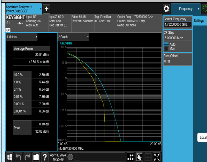
Band4-20MHz-16QAM-20175-1RB#0-PASS
