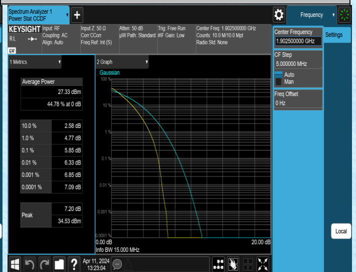
Band2-15MHz-QPSK-19125-75RB#0-PASS
