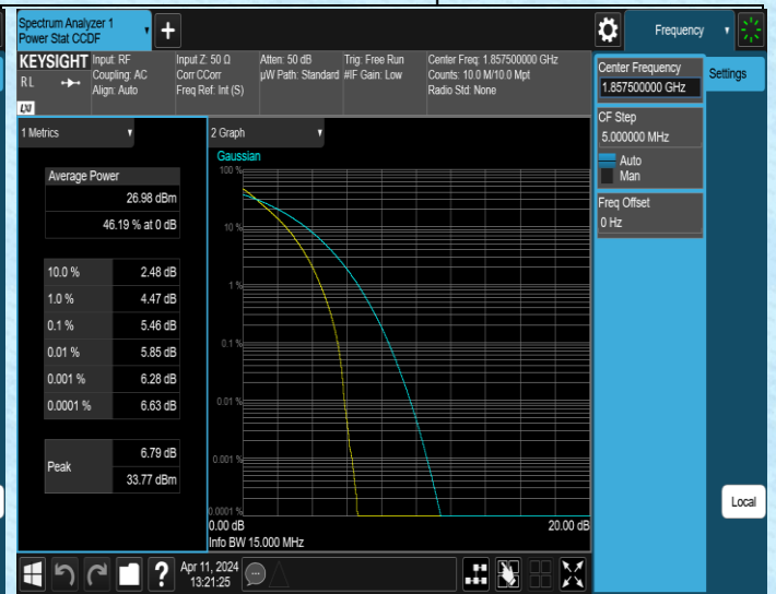
Band2-15MHz-QPSK-18675-75RB#0-PASS
