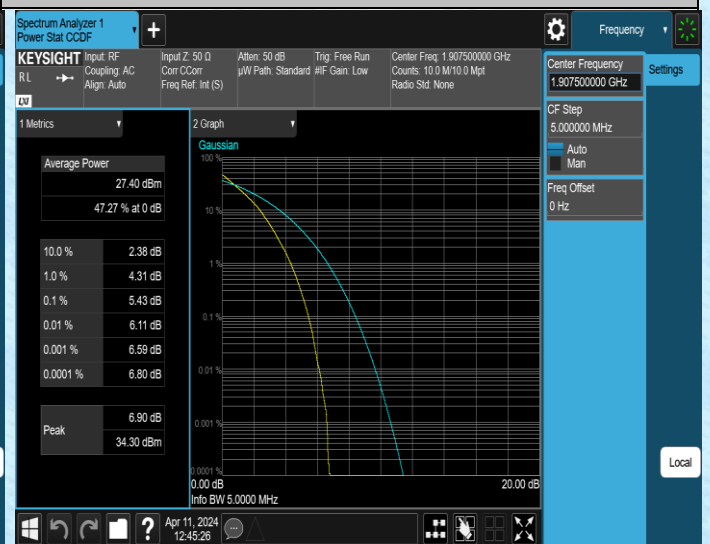
Band2-5MHz-QPSK-19175-25RB#0-PASS
