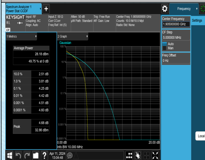
Band2-10MHz-QPSK-19150-1RB#0-PASS
