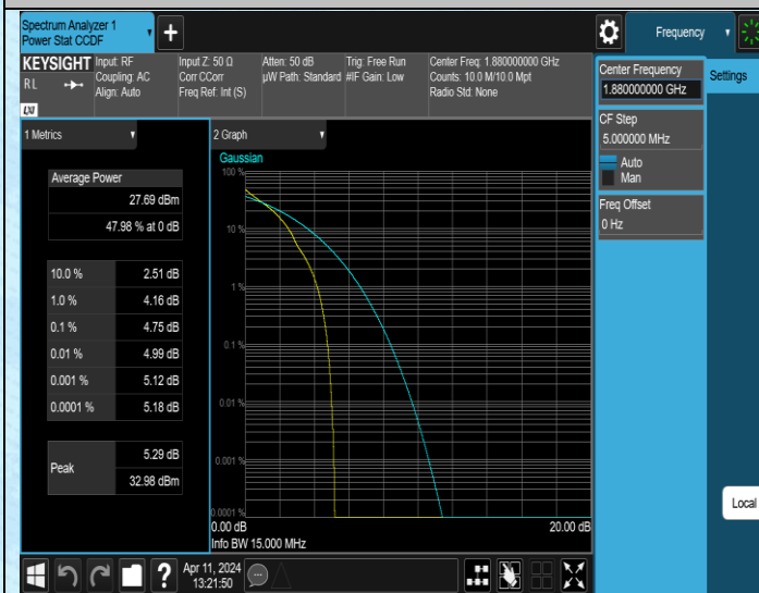
Band2-15MHz-QPSK-18900-1RB#0-PASS
