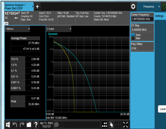
Band2-15MHz-QPSK-18675-1RB#0-PASS
