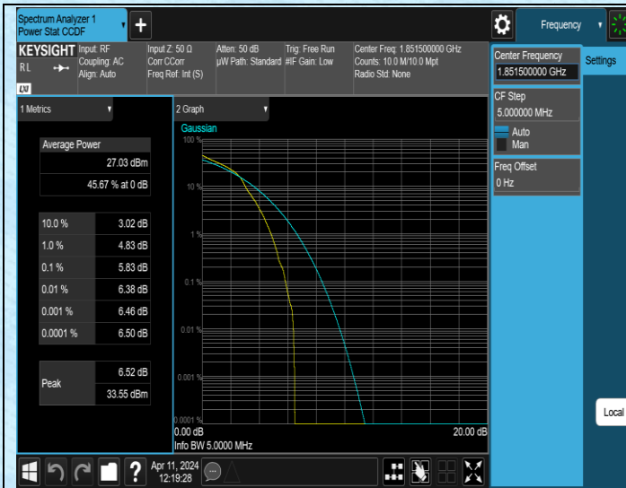
Band2-3MHz-16QAM-18615-1RB#0-PASS
