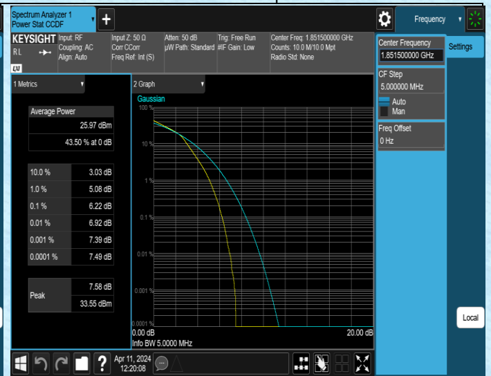
Band2-3MHz-16QAM-18615-15RB#0-PASS
