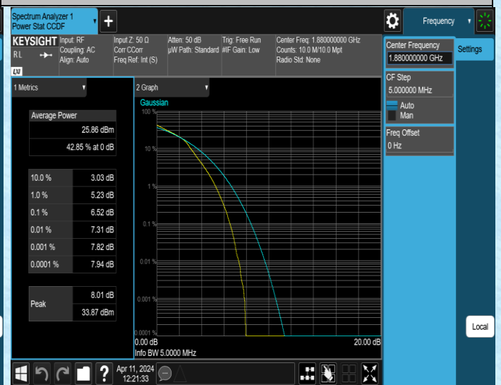
Band2-3MHz-16QAM-18900-15RB#0-PASS
