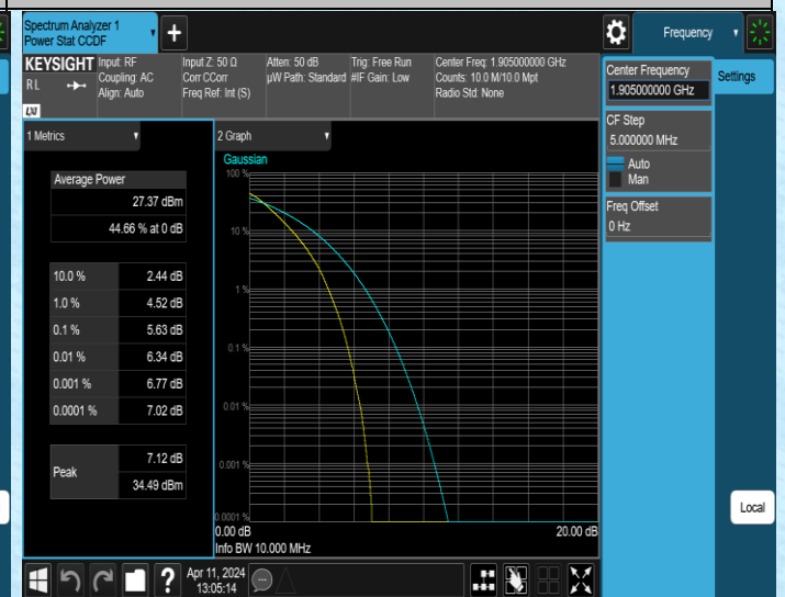
Band2-10MHz-QPSK-19150-50RB#0-PASS
