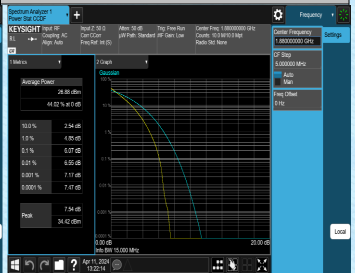
Band2-15MHz-QPSK-18900-75RB#0-PASS
