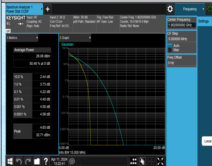
Band2-15MHz-QPSK-19125-1RB#0-PASS
