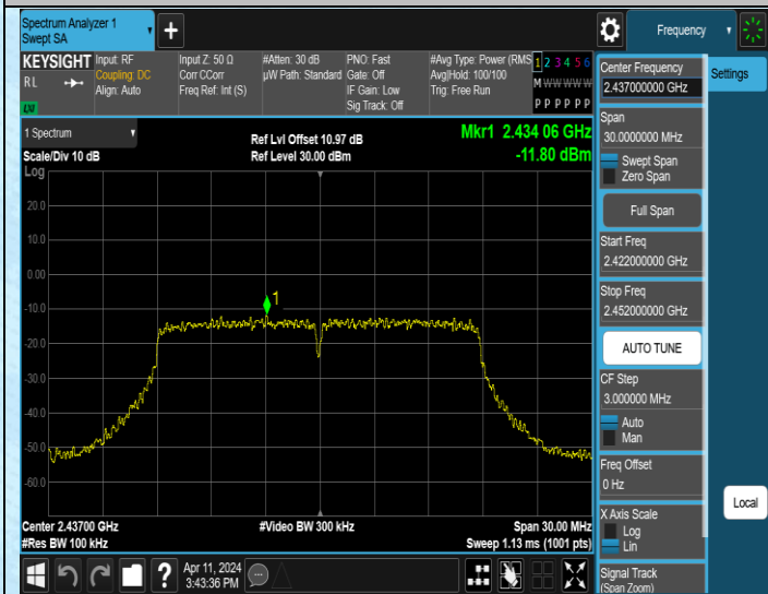
11N20MIMO-Ant1-2437-0~Reference-PASS
