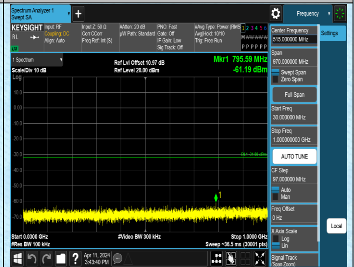
11N20MIMO-Ant1-2437-30~1000-PASS
