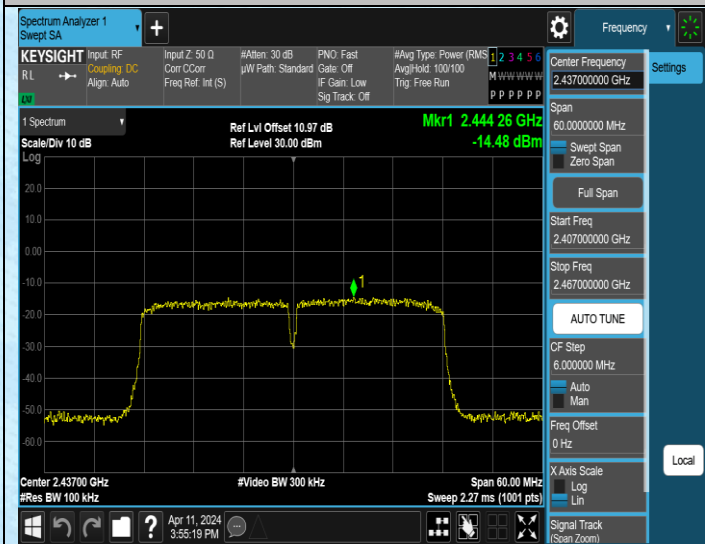
11N40MIMO-Ant1-2437-0~Reference-PASS
