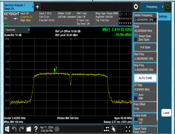
11N40MIMO-Ant2-2422-0~Reference-PASS
