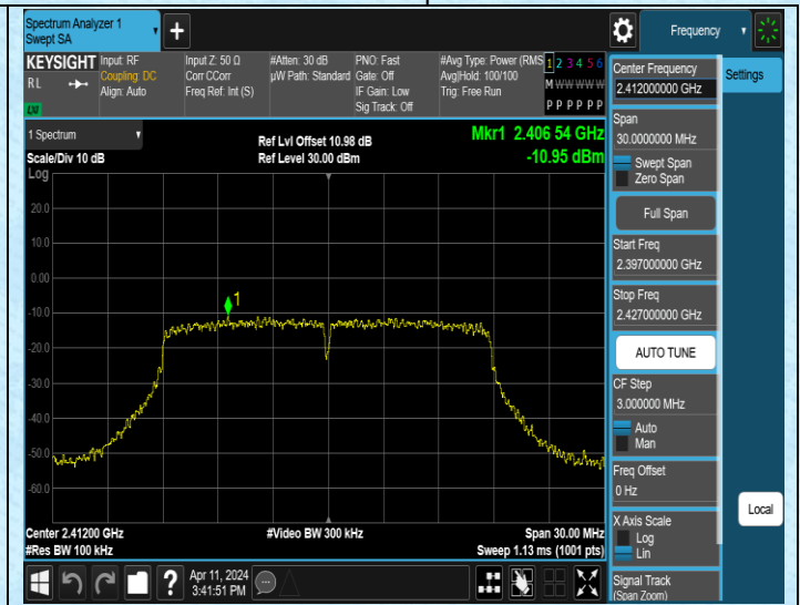
11N20MIMO-Ant2-2412-0~Reference-PASS
