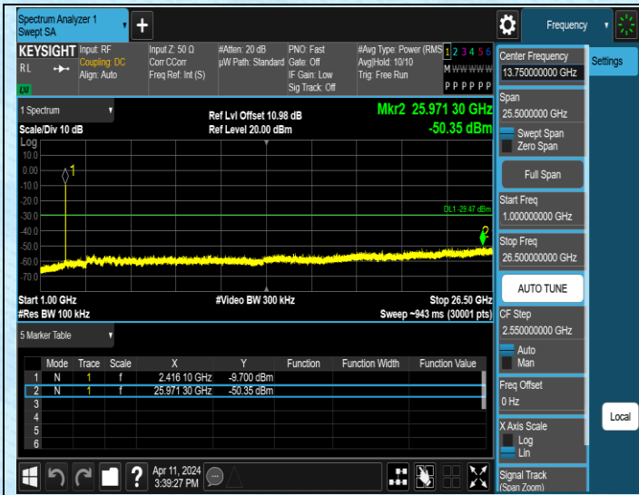
11N20MIMO-Ant1-2412-1000~26500-PASS
