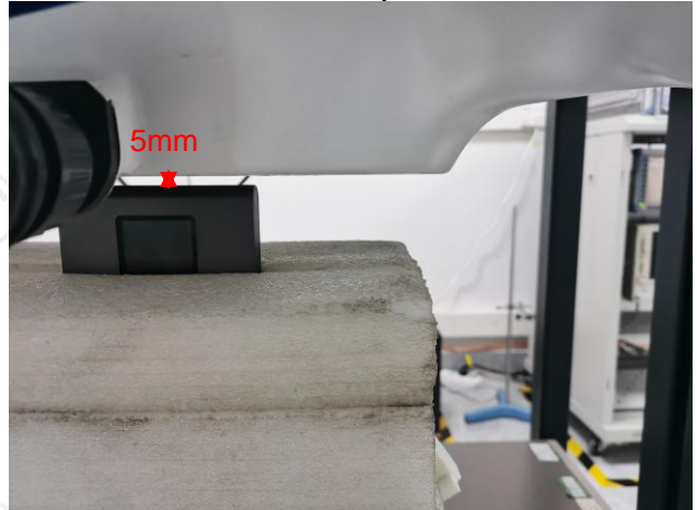
Hotspot Bottom(5mm)
