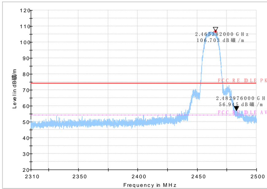
Peak detector
