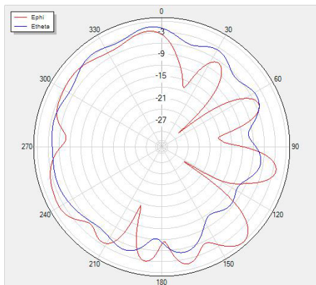
Phi=90 freq=2440MHz
