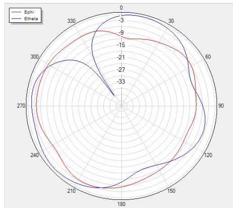
Phi=0 freq=2440MHz
