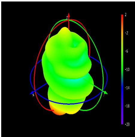
Phi=90 freq=2440MHz
