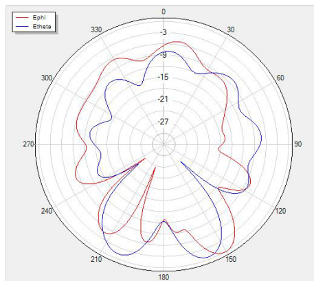
Phi=0 freq=2440MHz
