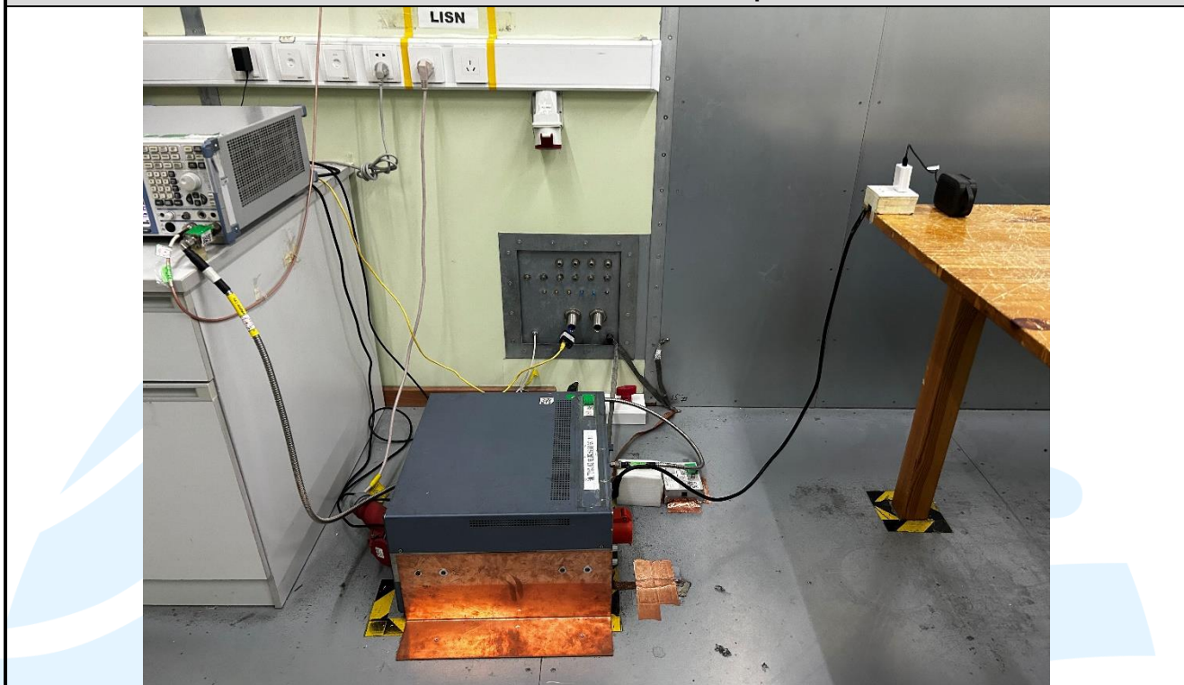
Conducted Emission Test Setup-3
