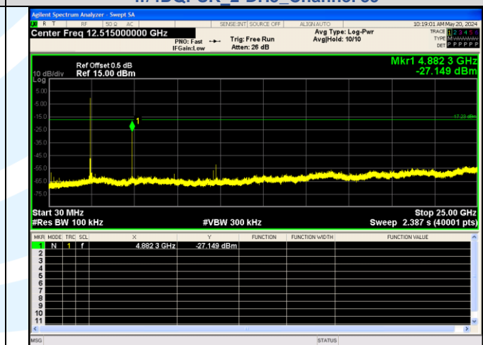
30.0 MHz - 25000.0 MHz \pi/4 DQPSK_2-DH5_Channel 39
