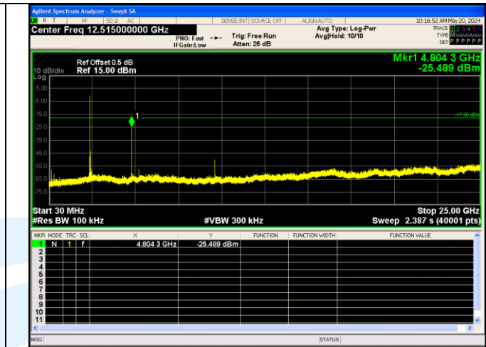
30.0 MHz - 25000.0 MHz \pi/4 DQPSK_2-DH5_Channel 0
