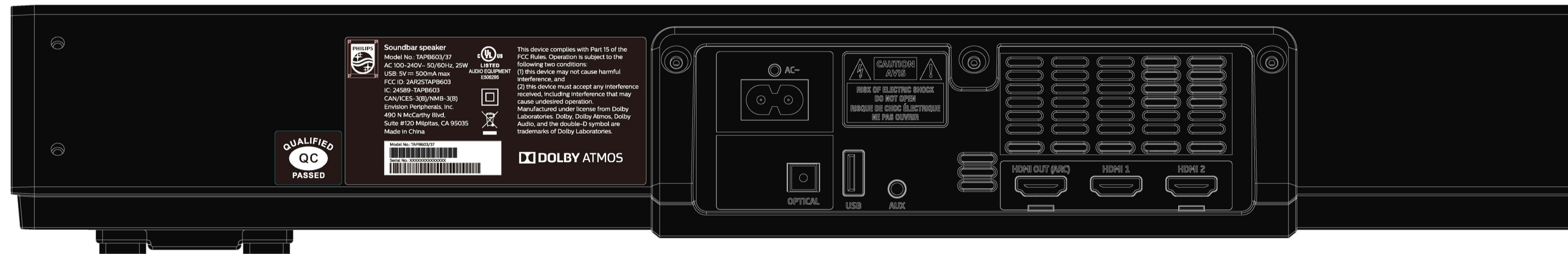
BACK VIEW-unit
