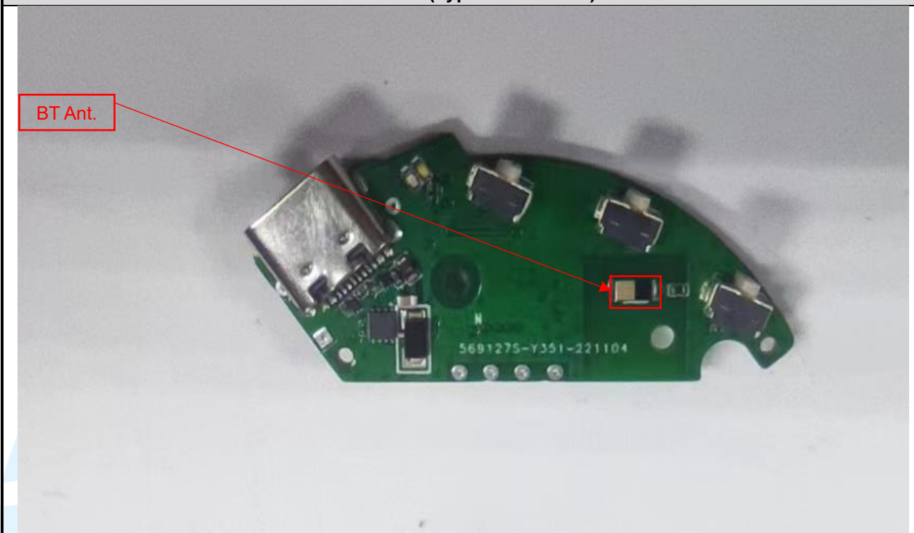
EUT Photo (Type A: With TVS)
