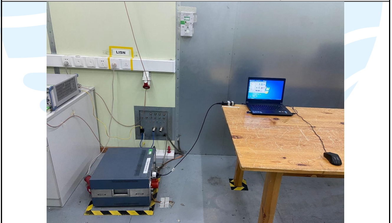
AC Power Line Conducted Emission Test Setup
