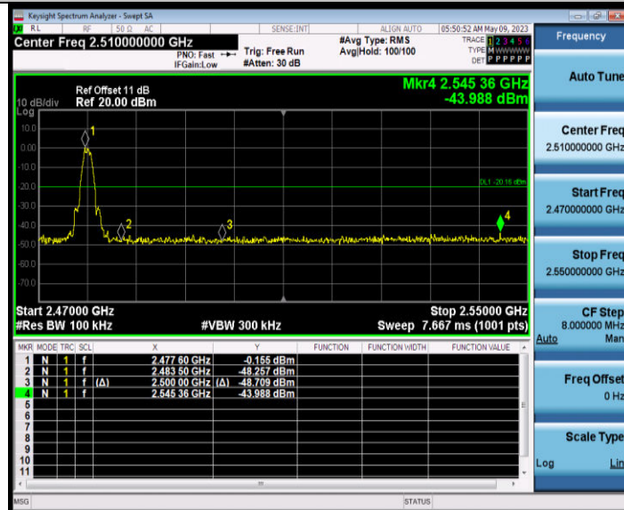
BLE_2M_Ant1_High_2478
