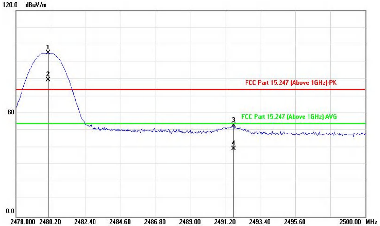
Antenna Polarity & Test Distance: Horizontal at 3 m
