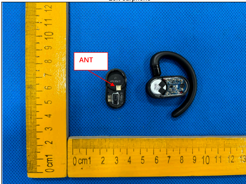
Left earphone
