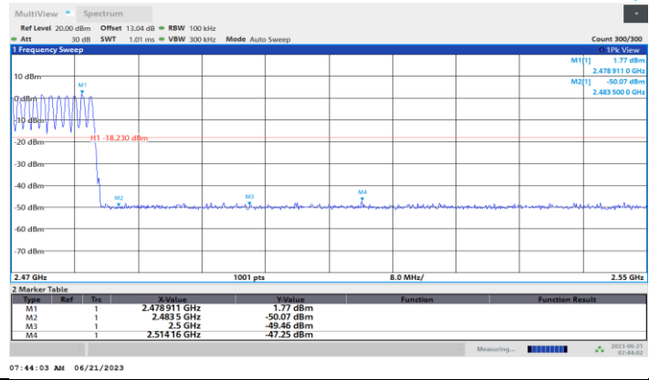
DH5_Ant1_High_Hop_2480
