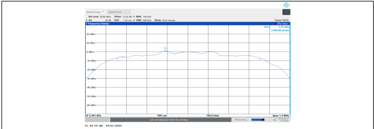
3DH5_Ant1_2441_0~Reference
