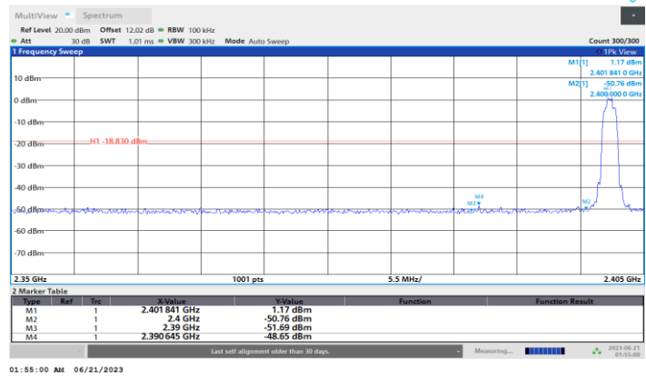
3DH5_Ant1_Low_2402
