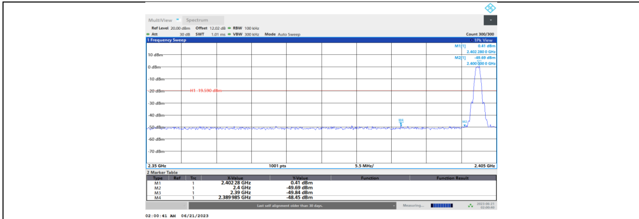
BLE_1M_Ant1_Low_2402
