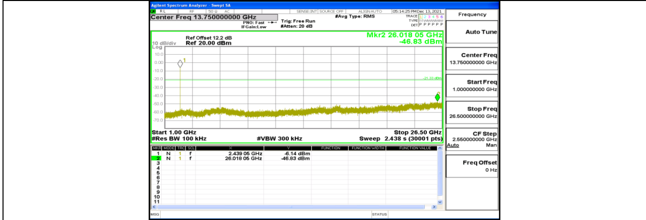
BLE_2M_Ant1_2440_1000~26500
