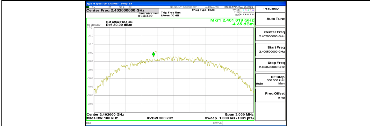
BLE_2M_Ant1_2402_0~Reference
