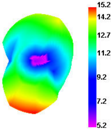
Bluetooth 39 TRP
