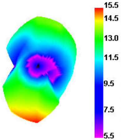
Bluetooth 0 TRP
