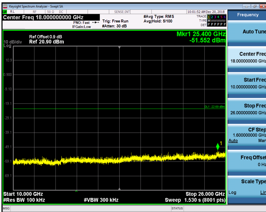
RF Conducted Spurious Emissions_2DH5_2480
