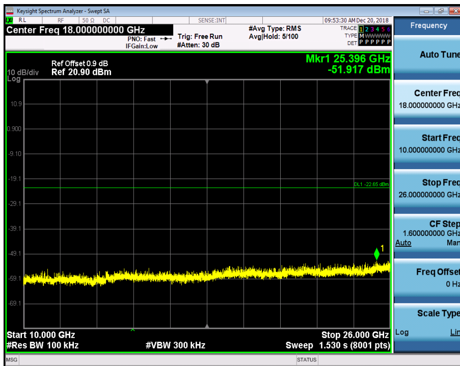
RF Conducted Spurious Emissions_2DH5_2402
