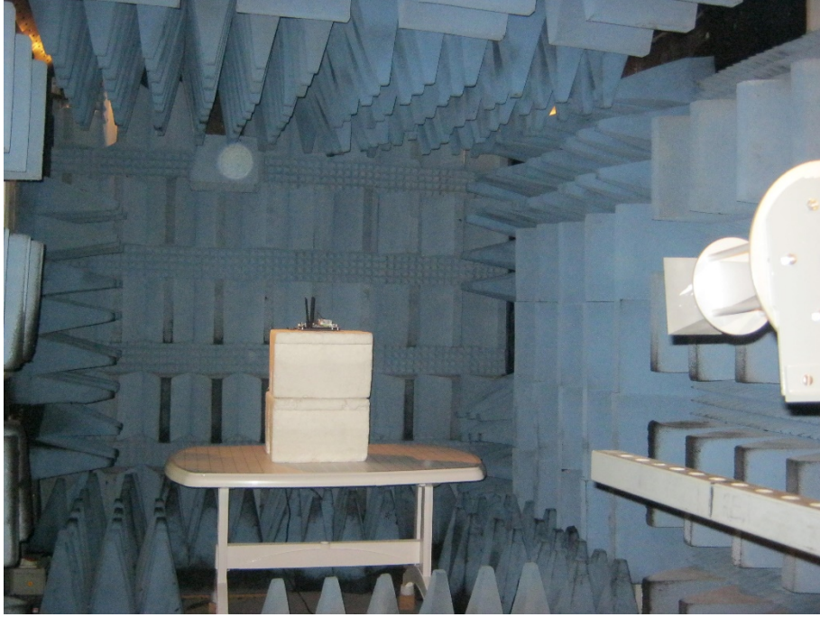
Figure 1. Radiated Emission Test Setup
