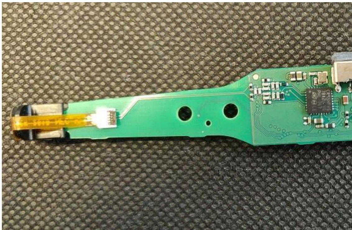
Close-up on NFC transceiver, matching network and coil.
