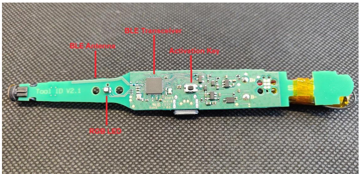
Top PCB view.
