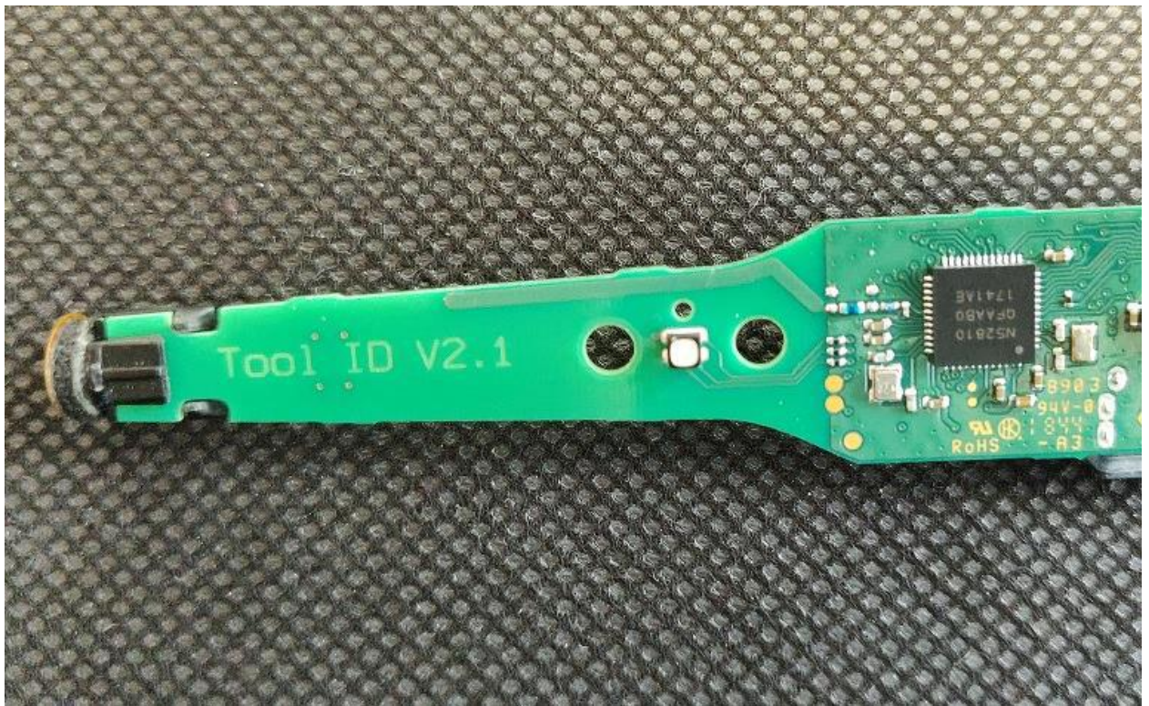
Close-up on BLE transceiver, matching network and antenna.
