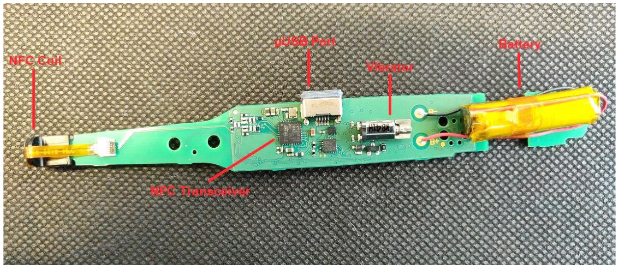
Bottom PCB view.
