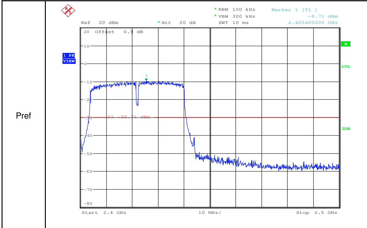
RF Conducted Spurious Emissions_11N40SISO_2422_Ant1
