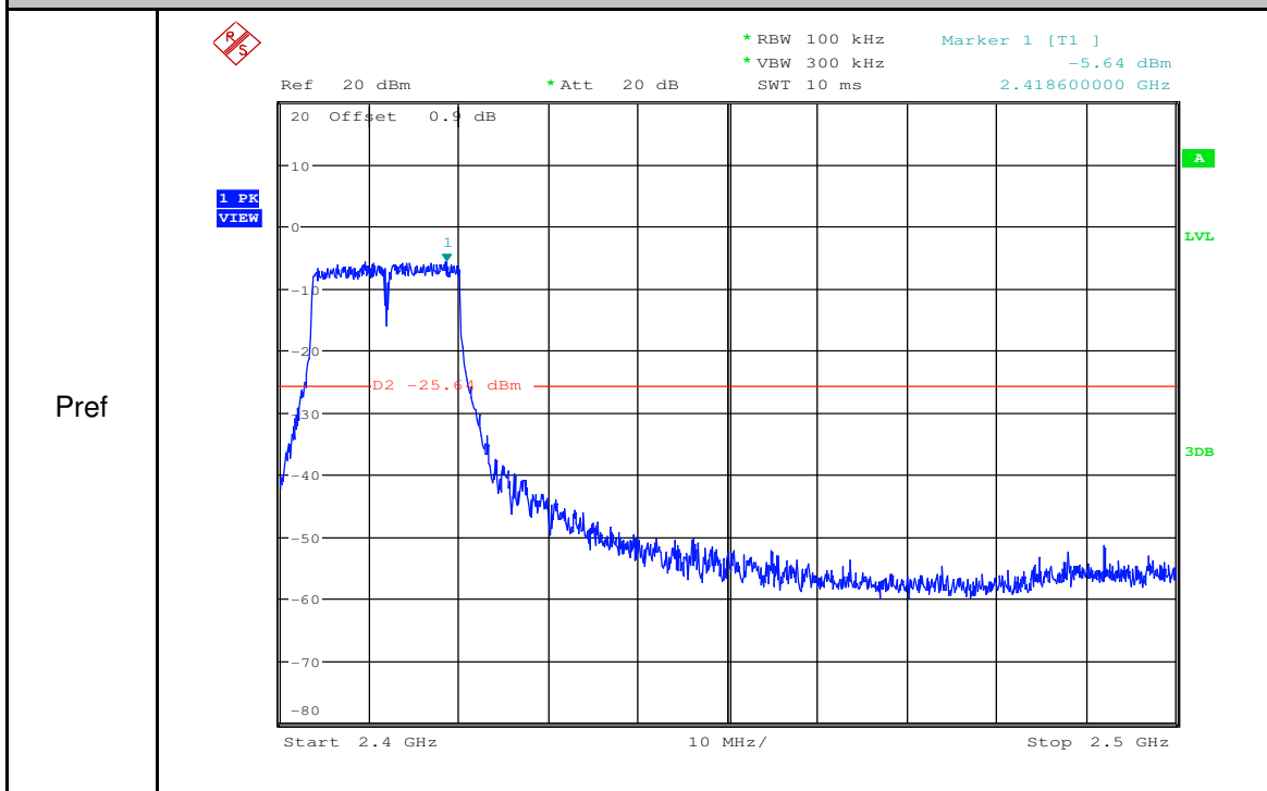
RF Conducted Spurious Emissions_11G_2412_Ant1
