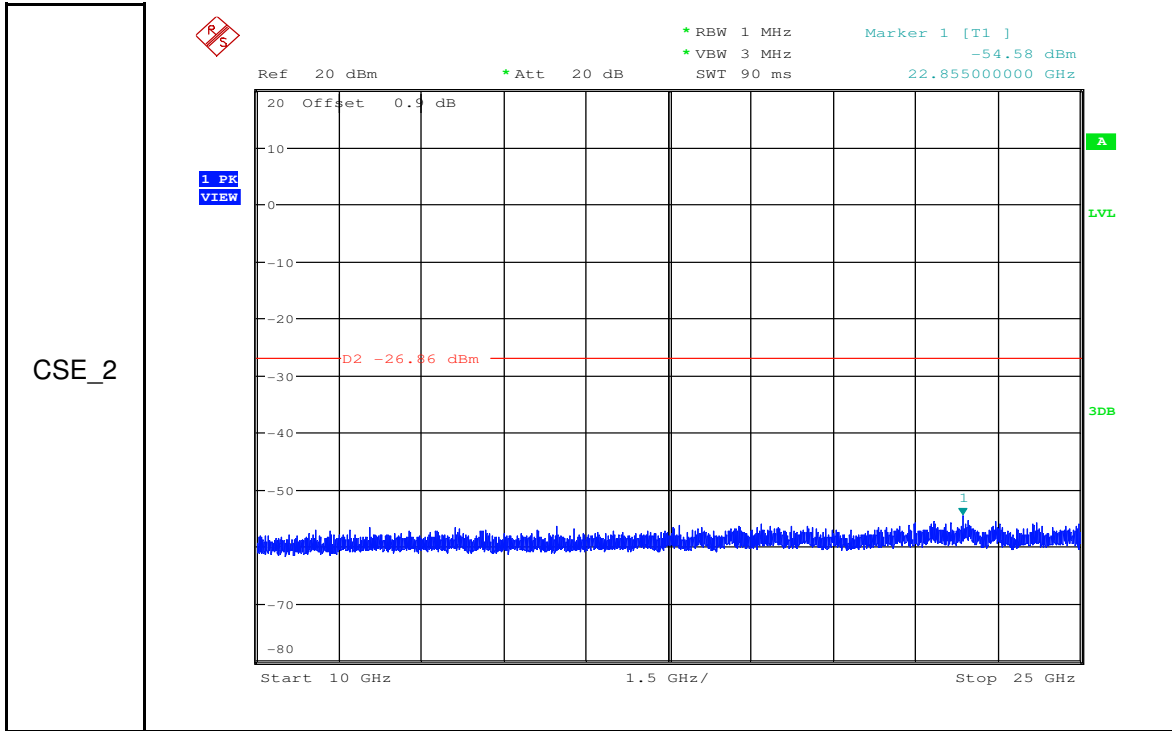
RF Conducted Spurious Emissions_11N20SISO_2437_Ant1
