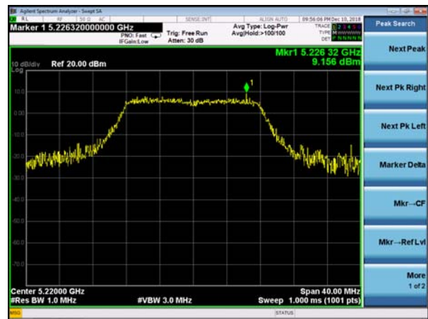
ANTB (5220 MHz) PSD plot on channel 01
