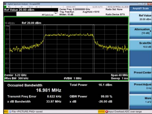
ANTB (5220MHz) -26dB&99%Bandwidth plot on channel 01
