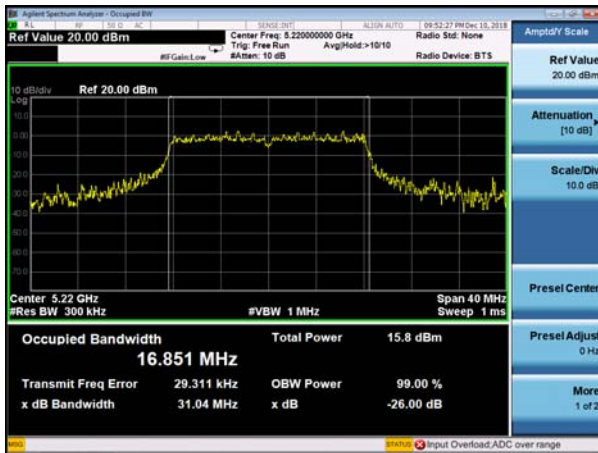
ANTA (5220MHz) -26dB&99%Bandwidth plot on channel 01
