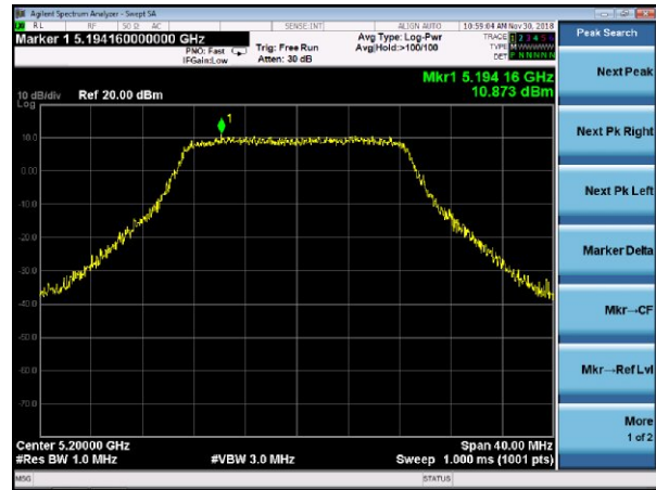
ANTB (5200 MHz) PSD plot on channel 01
