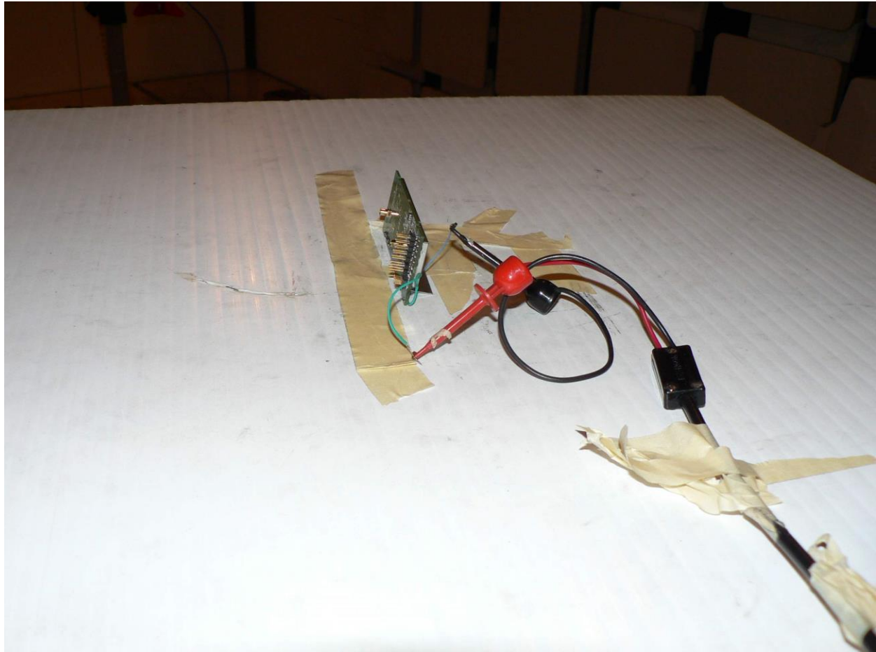
SHOO03 TX Spurious Closeup with Integral Antenna
