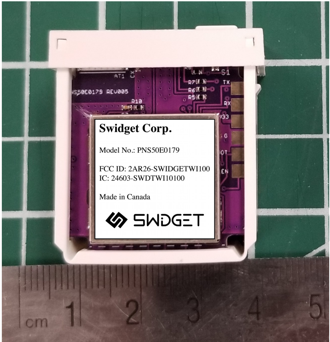
Figure 2: Bottom View
