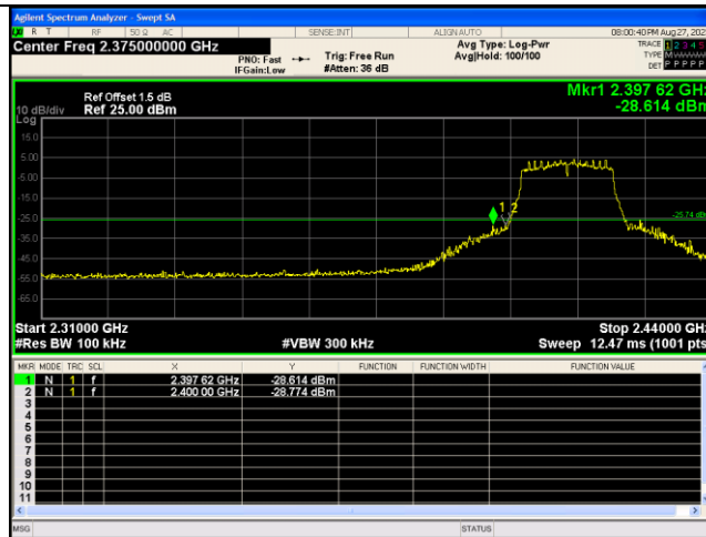
Out Of Band Emission IEEE 802.11n Channel 1 20MHz Antenna 0
