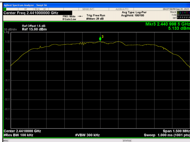
In-Band Reference Level 8DPSK 3-DH5 Channel 39
