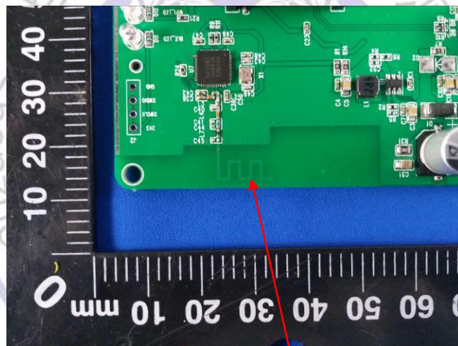
BT Antenna
