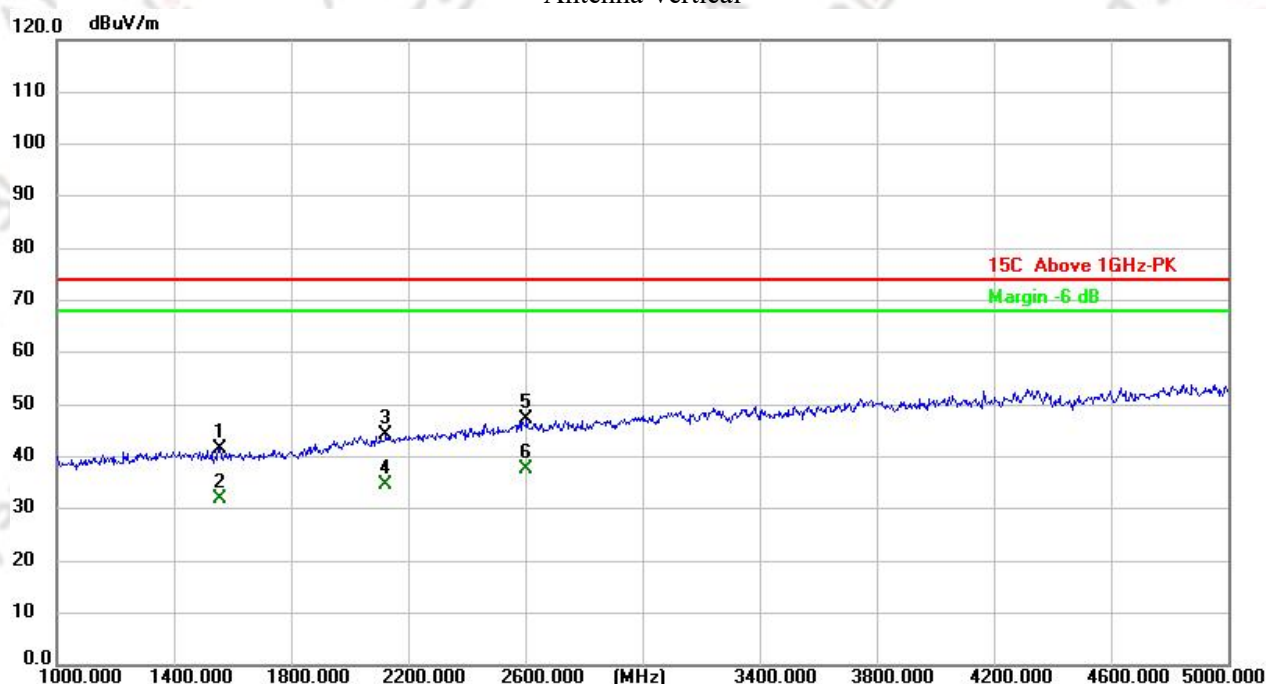
Antenna Vertical
