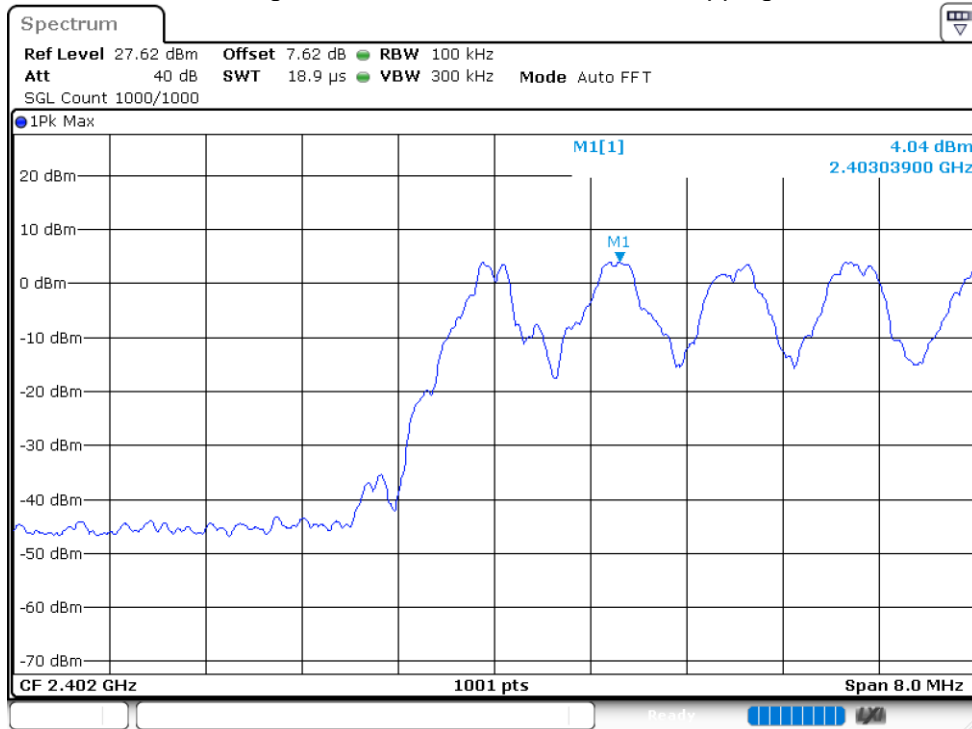
Band Edge NVNT 1-DH5 2402MHz Ant1 Hopping Ref
