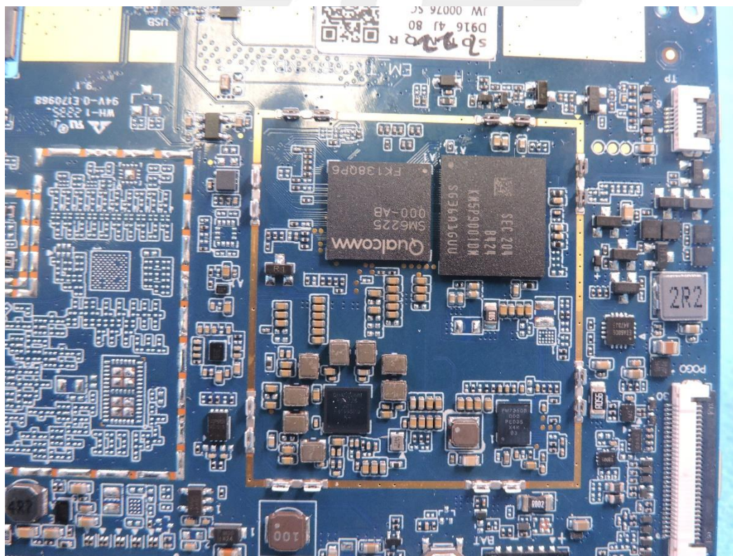
Photo 10 (Memory chip: Samsung KM5P9001DM)
