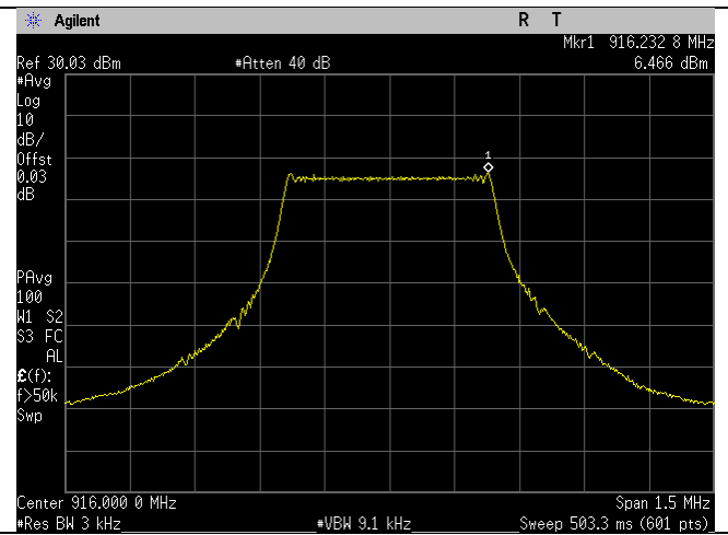
916MHz_Spectral Density_Lora1
