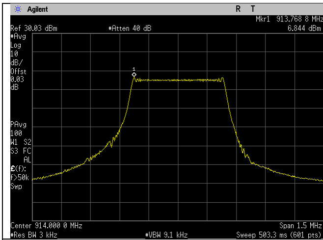
914MHz_Spectral Density_Lora1
