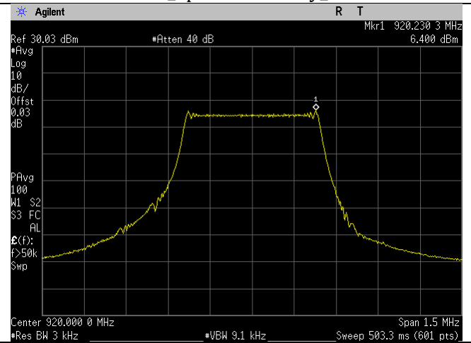
920MHz_Spectral Density_Lora2
