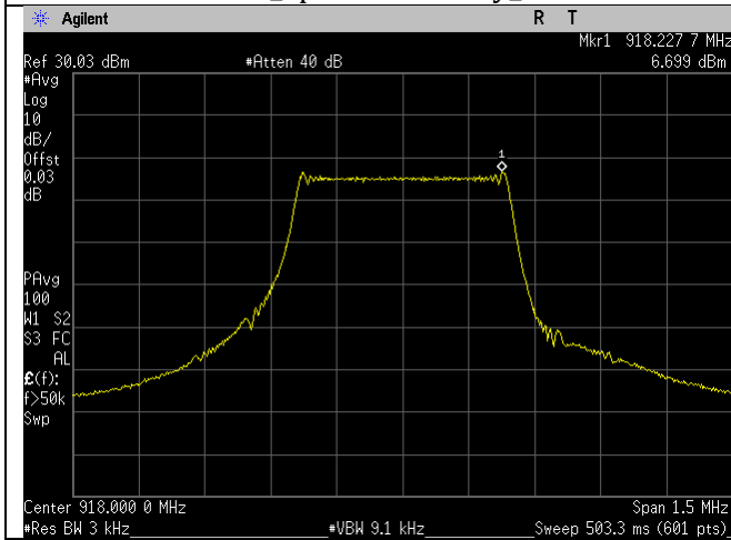
918MHz_Spectral Density_Lora1
