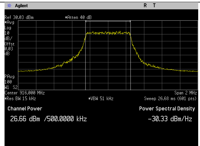
916MHz_Output Power_Lora1
