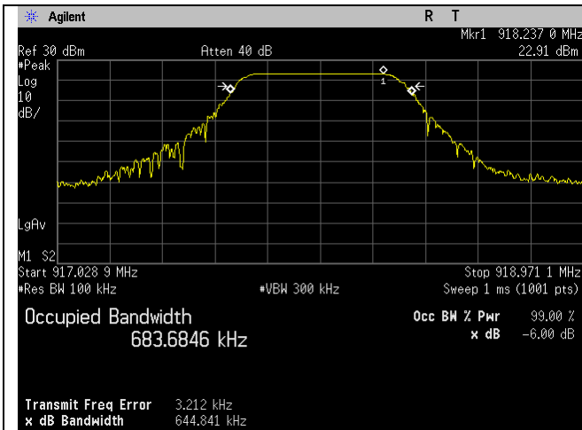
High Ch_918MHz_Occupied Bandwidth_-6dB_Lora 1
