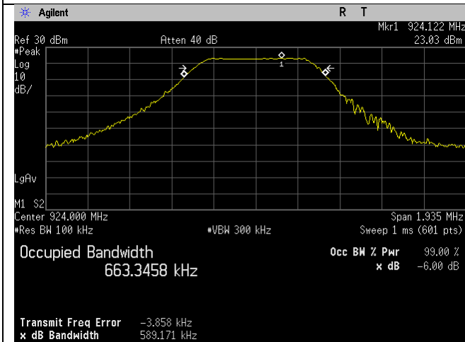
High Ch_924MHz_Occupied Bandwidth_-6dB_Lora 2
