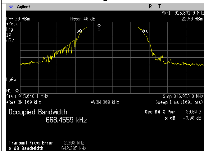
Mid Ch_916MHz_Occupied Bandwidth_-6dB_Lora 1
