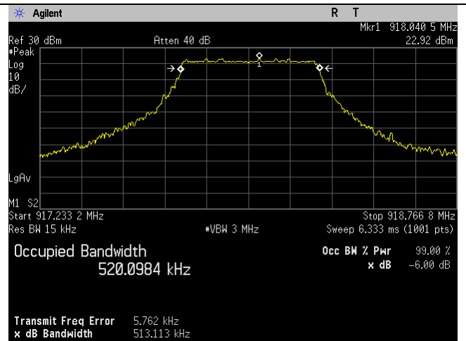
High Ch_918MHz_Occupied Bandwidth_99 percent_Lora 1
