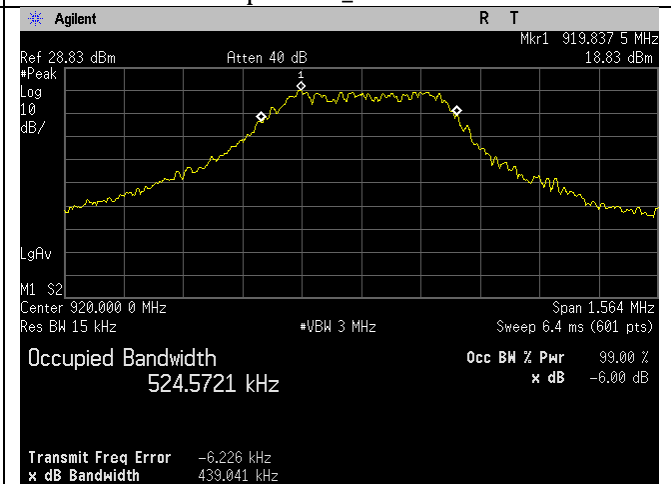
Low Ch_920MHz_Occupied Bandwidth_99 percent_Lora 2
