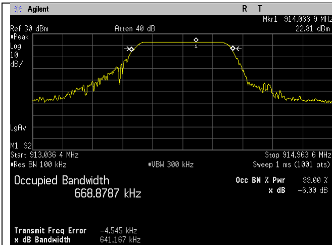
Low Ch_914MHz_Occupied Bandwidth_-6dB_Lora 1
