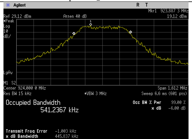
High Ch_924MHz_Occupied Bandwidth_99 percent_Lora 2
