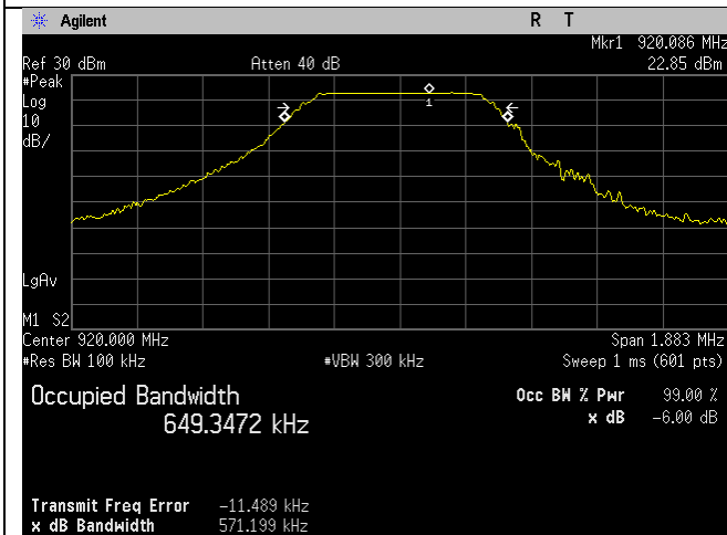
Low Ch_920MHz_Occupied Bandwidth_-6dB_Lora 2
