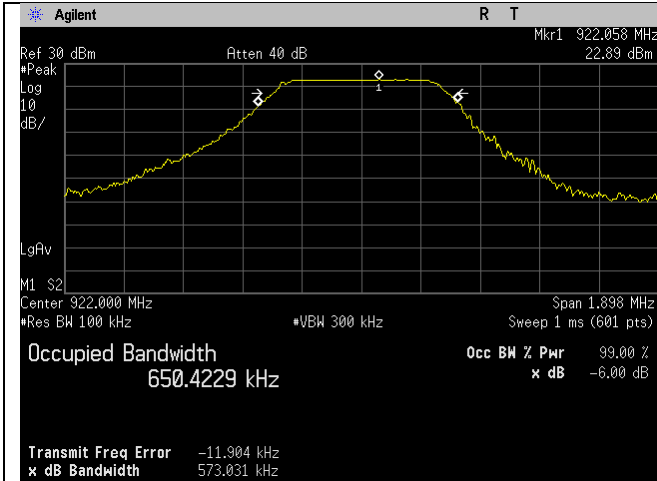
Mid Ch_922MHz_Occupied Bandwidth_-6dB_Lora 2
