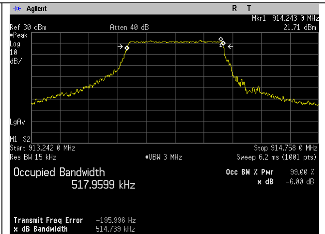
Low Ch_914MHz_Occupied Bandwidth_99 percent_Lora 1
