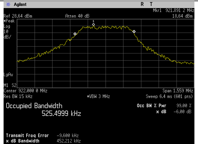
Mid Ch_922MHz_Occupied Bandwidth_99 percent_Lora 2
