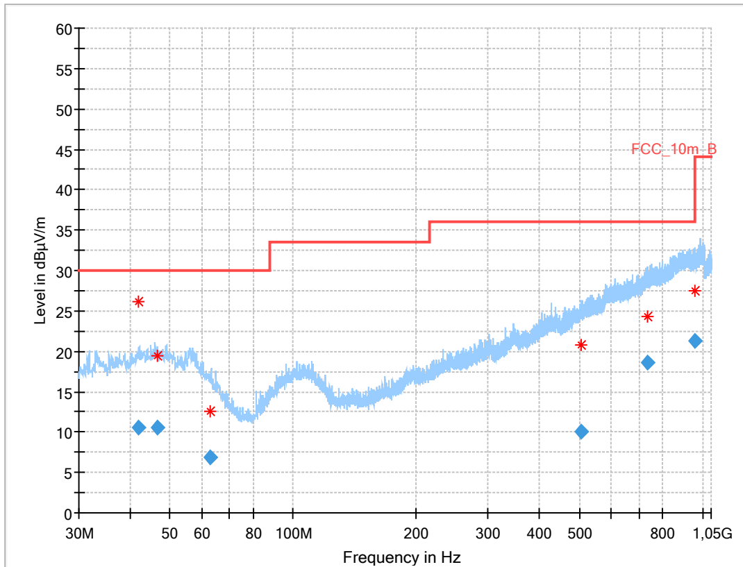
Plot 5: 30 MHz to 1 GHz, TX mode, 2440 MHz, vertical & horizontal polarization, 2 Msps, valid for all channels
