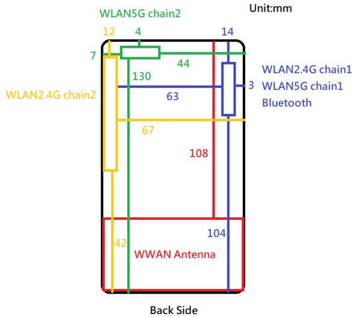
Fig.17 Antenna position of EUT
