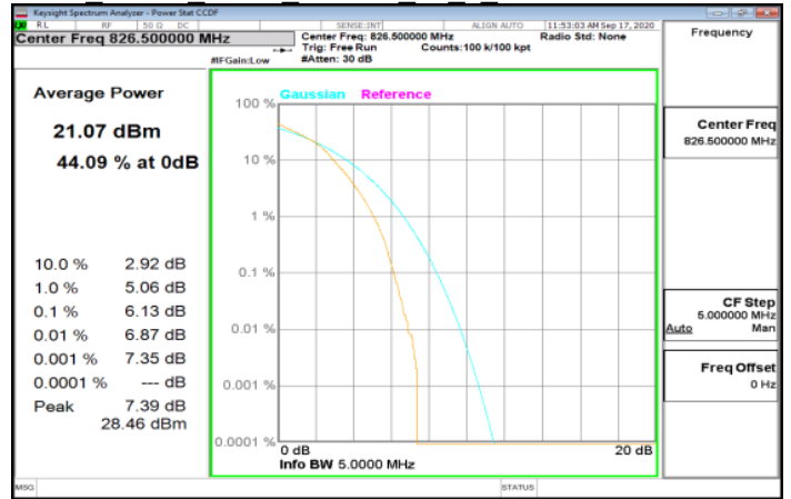
LTE Band5 5MHz 64QAM 25 0 LowCH20425-826.5
