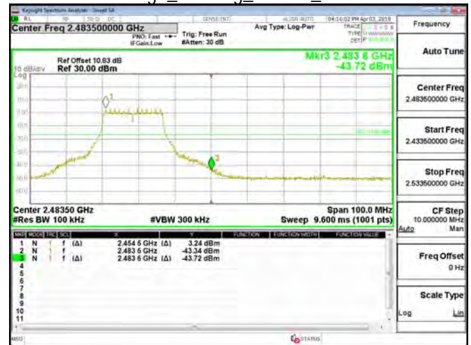
Band Edge_802.11g_20MHz_2462MHz
