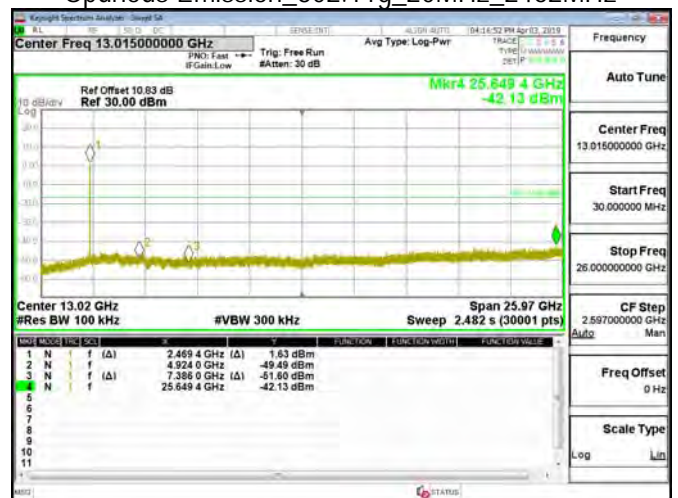
Spurious Emission_802.11g_20MHz_2462MHz
