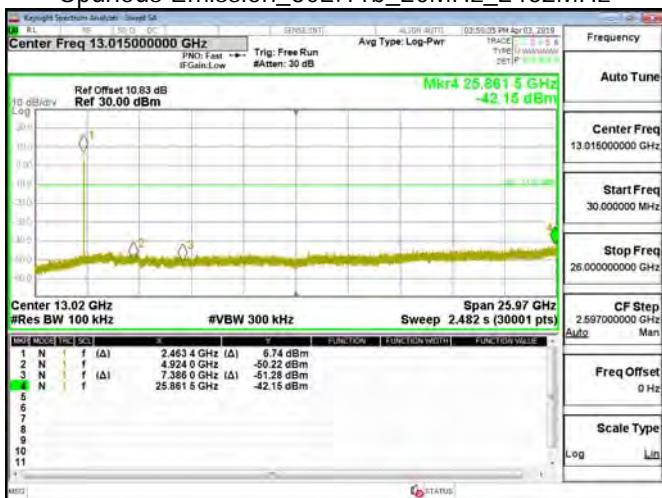
Spurious Emission_802.11b_20MHz_2462MHz
