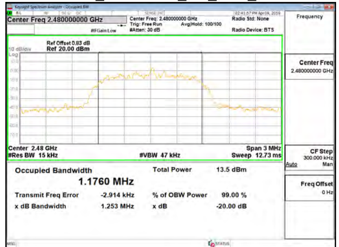
OBW 20dB_π4DQPSK_2M_DH5_2480MHz
