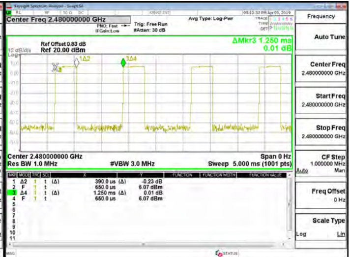
Dwell Time_π4DQPSK_2M_DH1_2480MHz
