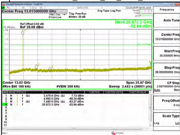
Spurious Emission_GFSK_1M_DH5_2480MHz
