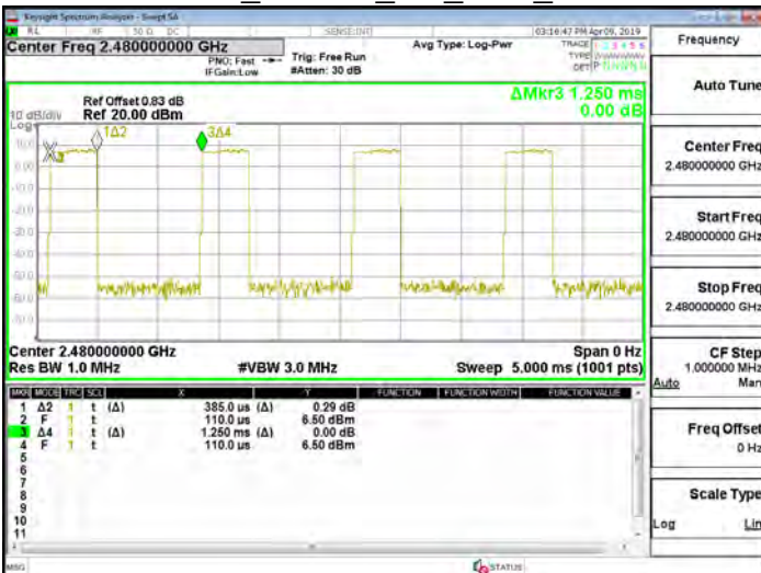
Dwell Time_8DPSK_3M_DH1_2480MHz
