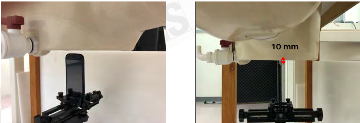
Fig.14 EUT Top side to flat phantom
