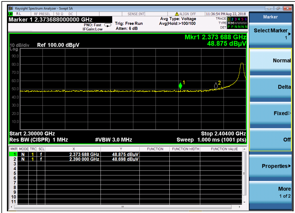
(Channel = 0, PEAK)
