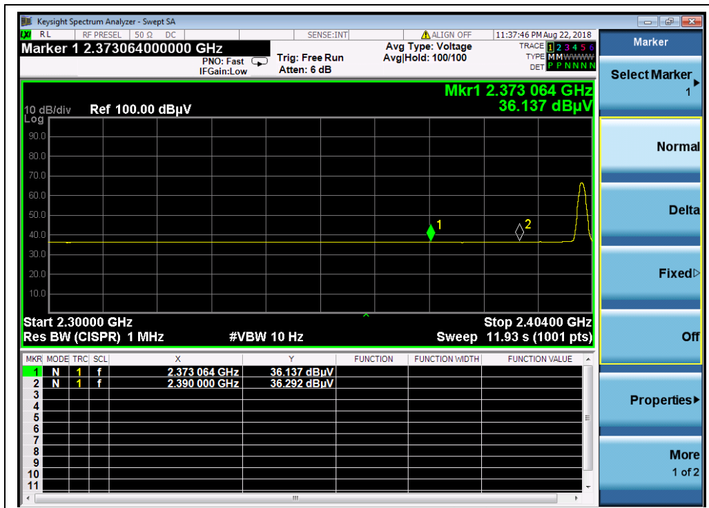
(Channel = 0, AVG)
