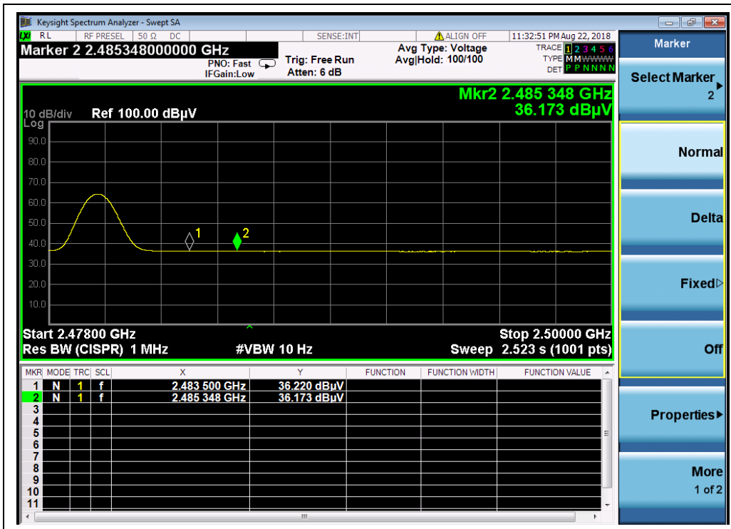
(Channel = 39, AVG)
