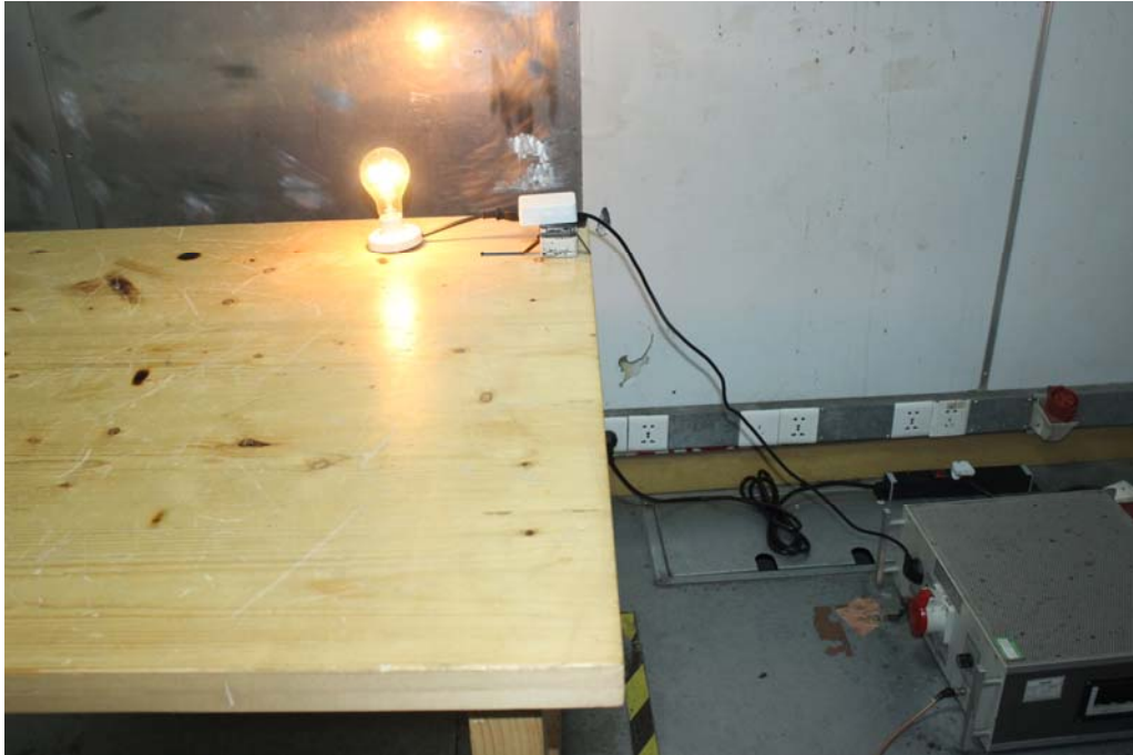
Photograph of set-up for ac power line Conducted emission
